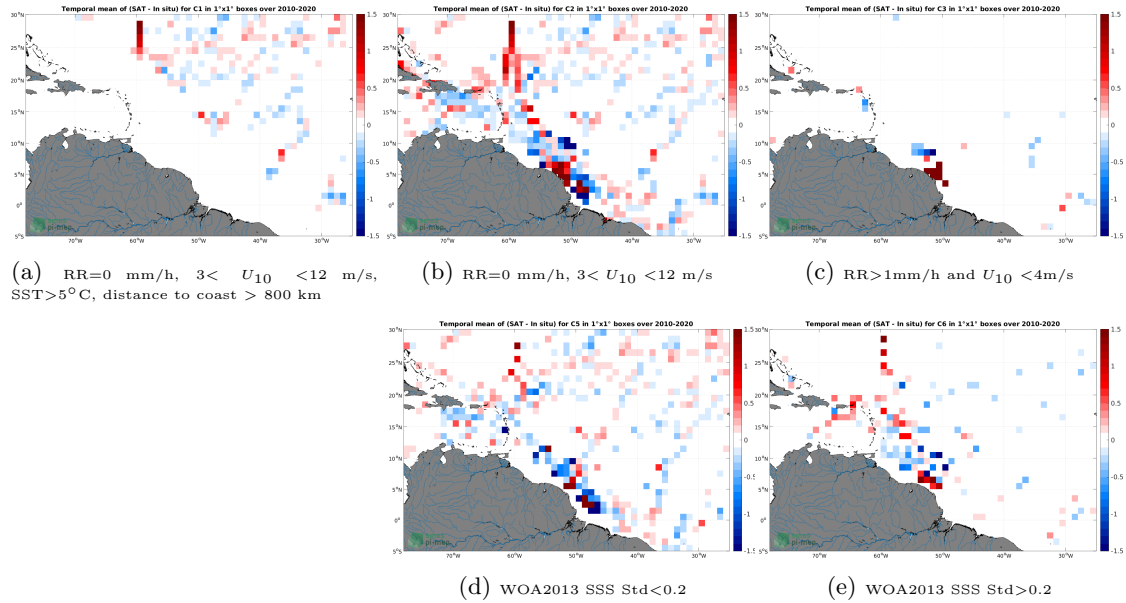
Figure 12: Temporal mean gridded over spatial boxes of size 1^{\circ}\times 1^{\circ} of \Delta SSS (SMOS SSS L3 v8 - 9 Days (CATDS-CECOS-LOCEAN) - TSG (GOSUD-Research-vessel)) for 5 different subdatasets corresponding to:RR=0 mm/h, 3 < U_{10} < 12 m/s, SST >5^{\circ}\text{C} , distance to coast > 800 km (a), RR=0 mm/h, 3 < U_{10} < 12 m/s (b), RR >1 mm/h and U_{10} < 4 m/s (c), WOA2013 SSS Std <0.2 (d), WOA2013 SSS Std >0.2 (e).
