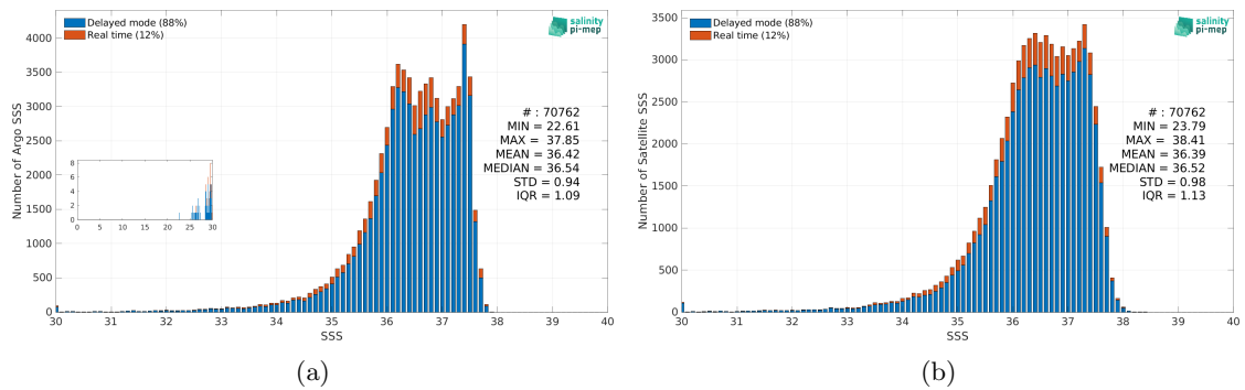
Figure 2: Histograms of SSS from Argo (a) and SMOS SSS L3 v8 - 9 Days (CATDS-CEC-LOCEAN) (b) considering all match-up pairs per bins of 0.1 over the Amazon and Orinoco river plumes Pi-MEP region and for the full satellite product period.
