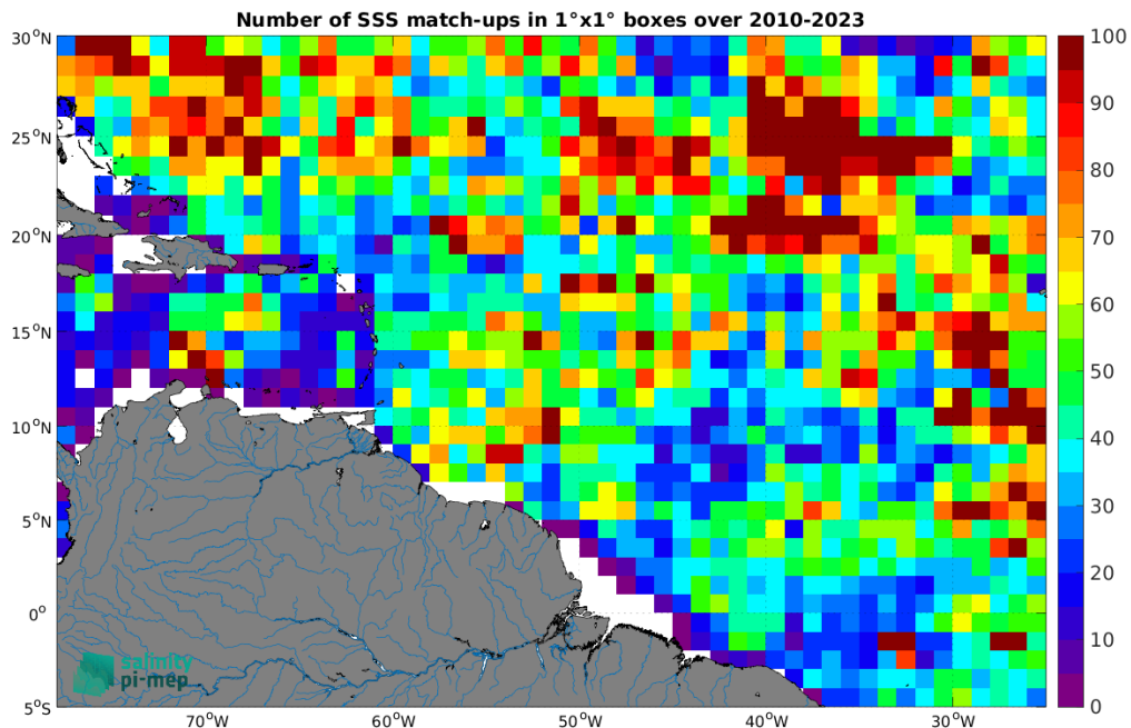
Figure 4: Number of SSS match-ups between Argo SSS and the SMOS SSS L3 v8 - 9 Days (CATDS-CEC-LOCEAN) SSS product for the Amazon and Orinoco river plumes Pi-MEP region over 1^\circ \times 1^\circ boxes and for the full satellite product period.
