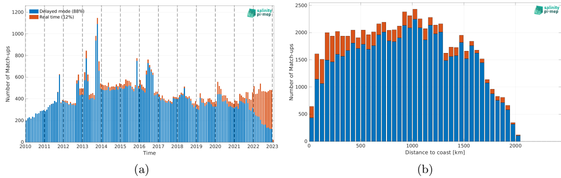
Figure 1: Number of match-ups between Argo and SMOS SSS L3 v8 - 9 Days (CATDS-CEC-LOCEAN) SSS as a function of time (a) and as function of the distance to coast (b) over the Amazon and Orinoco river plumes Pi-MEP region and for the full satellite product period.
