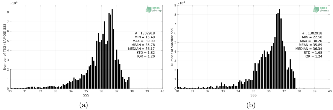
Figure 2: Histograms of SSS from TSG (SAMOS) (a) and SMOS SSS L3 v8 - 18 Days (CATDS-CECOS-LOCEAN) (b) considering all match-up pairs per bins of 0.1 over the Amazon and Orinoco river plumes Pi-MEP region and for the full satellite product period.
