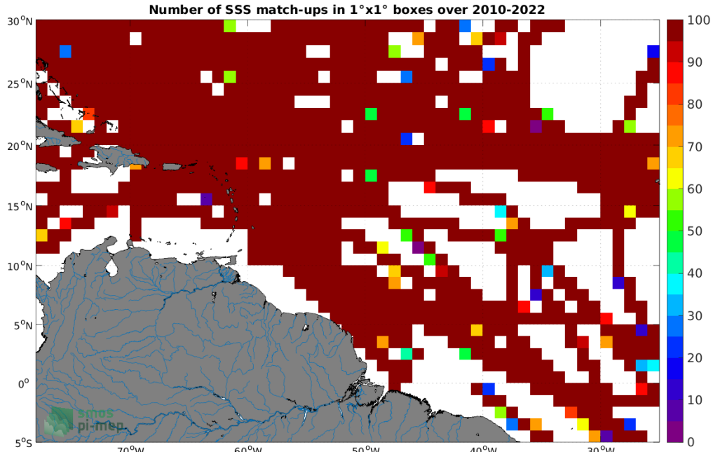
Figure 4: Number of SSS match-ups between TSG (SAMOS) SSS and the SMOS SSS L3 v8 - 18 Days (CATDS-CECOS-LOCEAN) SSS product for the Amazon and Orinoco river plumes Pi-MEP region over 1^\circ \times 1^\circ boxes and for the full satellite product period.
