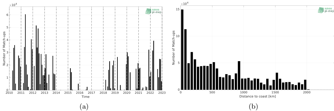
Figure 1: Number of match-ups between TSG (SAMOS) and SMOS SSS L3 v8 - 18 Days (CATDS-CECOS-LOCEAN) SSS as a function of time (a) and as function of the distance to coast (b) over the Amazon and Orinoco river plumes Pi-MEP region and for the full satellite product period.
