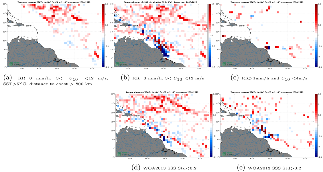
Figure 12: Temporal mean gridded over spatial boxes of size 1^{\circ}\times 1^{\circ} of \Delta\text{SSS} (SMOS SSS L3 v8 - 18 Days (CATDS-CECOS-LOCEAN) - TSG (SAMOS)) for 5 different subdatasets corresponding to:RR=0 mm/h, 3 < U_{10} < 12 m/s, SST >5^{\circ}\text{C} , distance to coast > 800 km (a), RR=0 mm/h, 3 < U_{10} < 12 m/s (b), RR >1 mm/h and U_{10} < 4 m/s (c), WOA2013 SSS Std <0.2 (d), WOA2013 SSS Std >0.2 (e).
