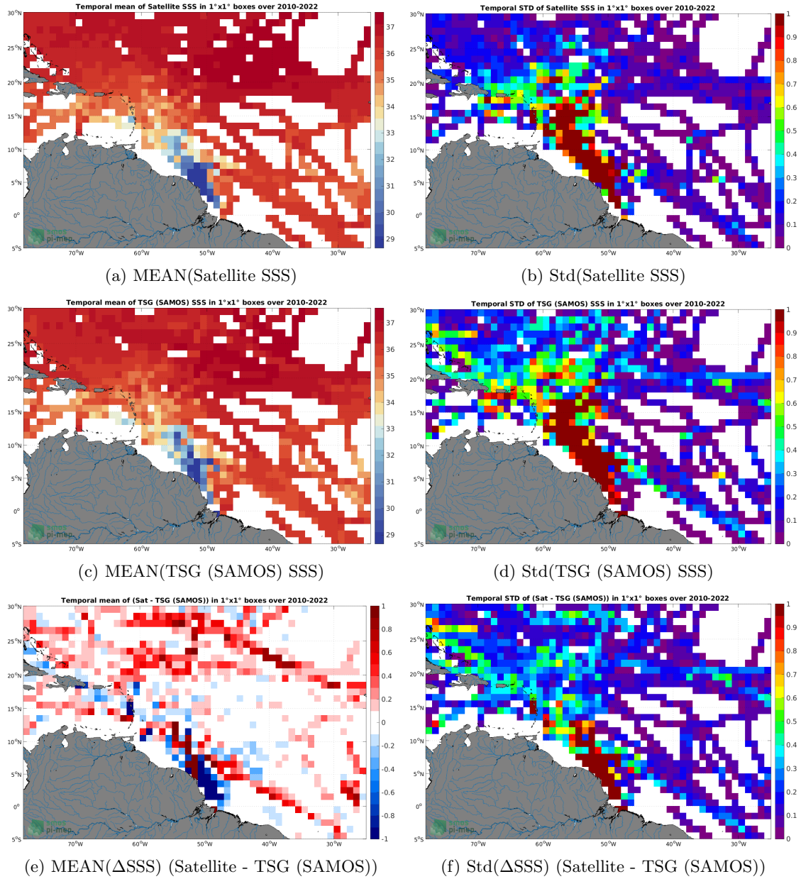
Figure 6: Temporal mean (left) and Std (right) of SSS from SMOS SSS L3 v8 - 18 Days (CATDS-CECOS-LOCEAN) (top), TSG (SAMOS) (middle), and of \Delta SSS (Satellite - TSG (SAMOS)). Only match-up pairs are used to generate these maps.
