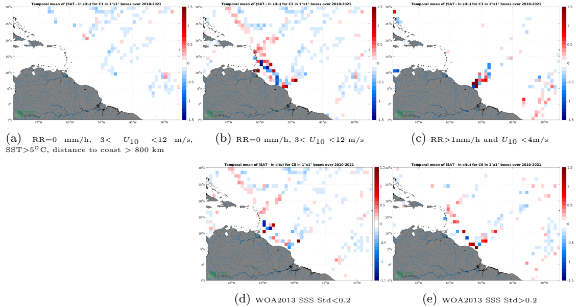
Figure 12: Temporal mean gridded over spatial boxes of size 1^{\circ}\times 1^{\circ} of \Delta\text{SSS} (SMOS SSS L3 v8 - 18 Days (CATDS-CECOS-LOCEAN) - TSG (LEGOS-DM)) for 5 different subdatasets corresponding to:RR=0 mm/h, 3 < U_{10} < 12 m/s, SST >5^{\circ}\text{C} , distance to coast > 800 km (a), RR=0 mm/h, 3 < U_{10} < 12 m/s (b), RR >1 mm/h and U_{10} < 4 m/s (c), WOA2013 SSS Std <0.2 (d), WOA2013 SSS Std >0.2 (e).
