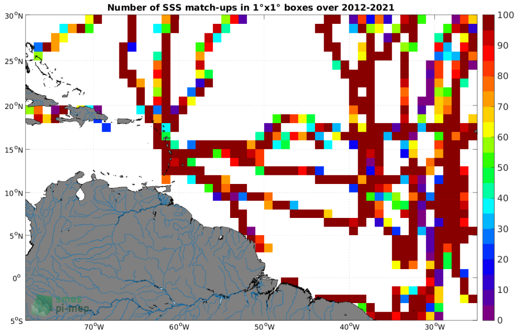
Figure 4: Number of SSS match-ups between TSG (GOSUD-Sailing-ship) SSS and the SMOS SSS L3 v8 - 18 Days (CATDS-CECOS-LOCEAN) SSS product for the Amazon and Orinoco river plumes Pi-MEP region over 1^\circ \times 1^\circ boxes and for the full satellite product period.
