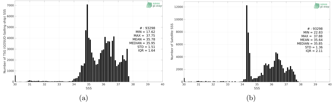
Figure 2: Histograms of SSS from TSG (GOSUD-Sailing-ship) (a) and SMOS SSS L3 v8 - 18 Days (CATDS-CECOS-LOCEAN) (b) considering all match-up pairs per bins of 0.1 over the Amazon and Orinoco river plumes Pi-MEP region and for the full satellite product period.
