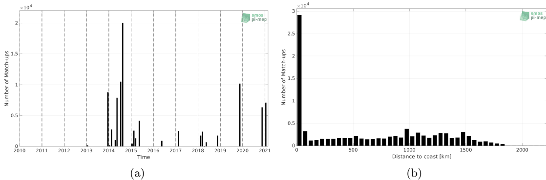
Figure 1: Number of match-ups between TSG (GOSUD-Sailing-ship) and SMOS SSS L3 v8 - 18 Days (CATDS-CECOS-LOCEAN) SSS as a function of time (a) and as function of the distance to coast (b) over the Amazon and Orinoco river plumes Pi-MEP region and for the full satellite product period.
