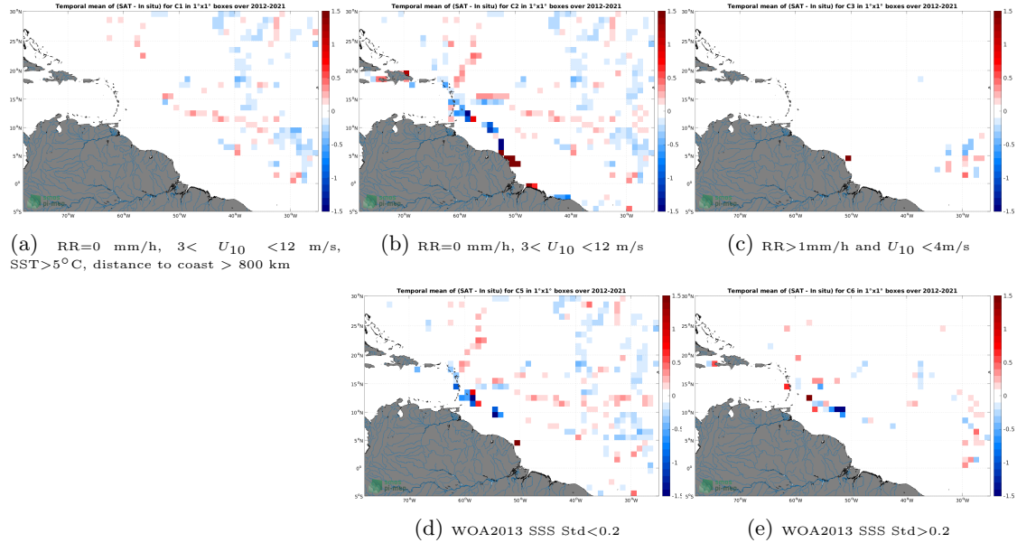
Figure 12: Temporal mean gridded over spatial boxes of size 1^{\circ}\times 1^{\circ} of \Delta SSS (SMOS SSS L3 v8 - 18 Days (CATDS-CECOS-LOCEAN) - TSG (GOSUD-Sailing-ship)) for 5 different subdatasets corresponding to:RR=0 mm/h, 3 < U_{10} < 12 m/s, SST >5^{\circ}\text{C} , distance to coast > 800 km (a), RR=0 mm/h, 3 < U_{10} < 12 m/s (b), RR >1 mm/h and U_{10} < 4 m/s (c), WOA2013 SSS Std <0.2 (d), WOA2013 SSS Std >0.2 (e).
