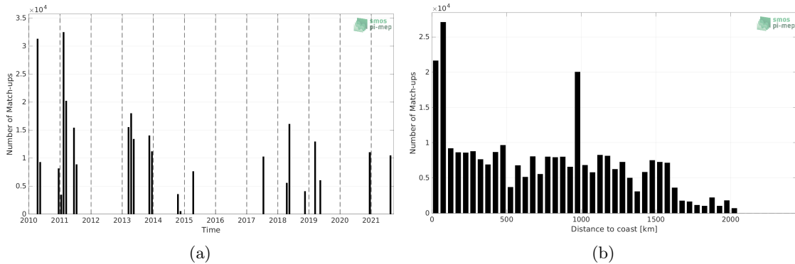
Figure 1: Number of match-ups between TSG (CSIC-UTM) and SMOS SSS L3 v8 - 18 Days (CATDS-CECOS-LOCEAN) SSS as a function of time (a) and as function of the distance to coast (b) over the Amazon and Orinoco river plumes Pi-MEP region and for the full satellite product period.
