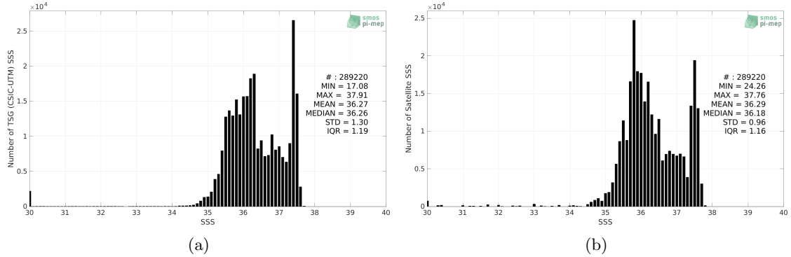
Figure 2: Histograms of SSS from TSG (CSIC-UTM) (a) and SMOS SSS L3 v8 - 18 Days (CATDS-CECOS-LOCEAN) (b) considering all match-up pairs per bins of 0.1 over the Amazon and Orinoco river plumes Pi-MEP region and for the full satellite product period.
