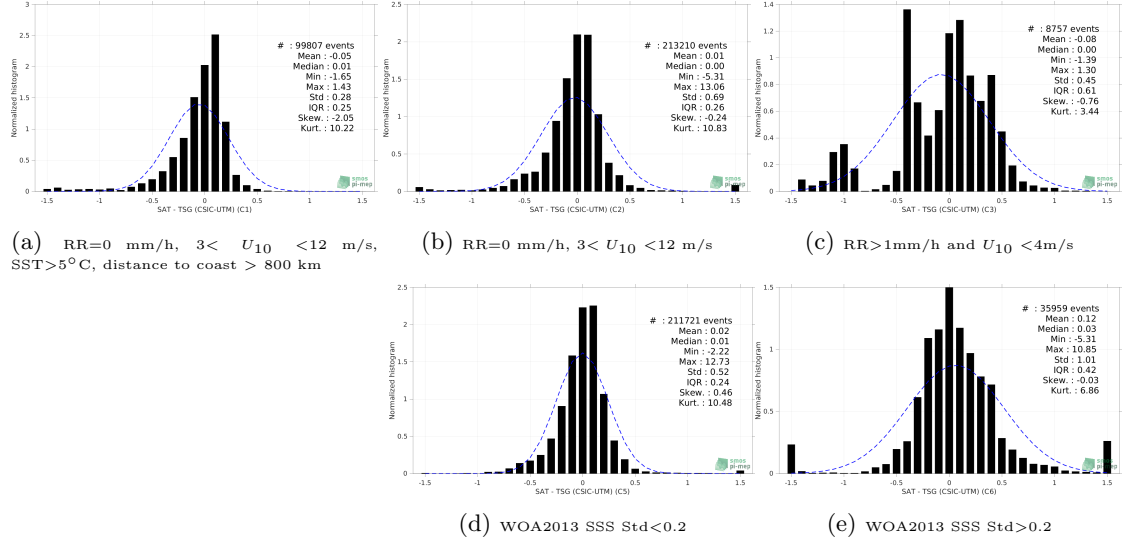
Figure 13: Normalized histogram of \Delta\text{SSS} (SMOS SSS L3 v8 - 18 Days (CATDS-CECOS-LOCEAN) - TSG (CSIC-UTM)) for 5 different subdatasets corresponding to: RR=0 mm/h, 3 < U_{10} < 12 m/s, SST>5°C, distance to coast > 800 km (a), RR=0 mm/h, 3 < U_{10} < 12 m/s (b), RR>1mm/h and U_{10} < 4 m/s (c), WOA2013 SSS Std<0.2 (d), WOA2013 SSS Std>0.2 (e).
