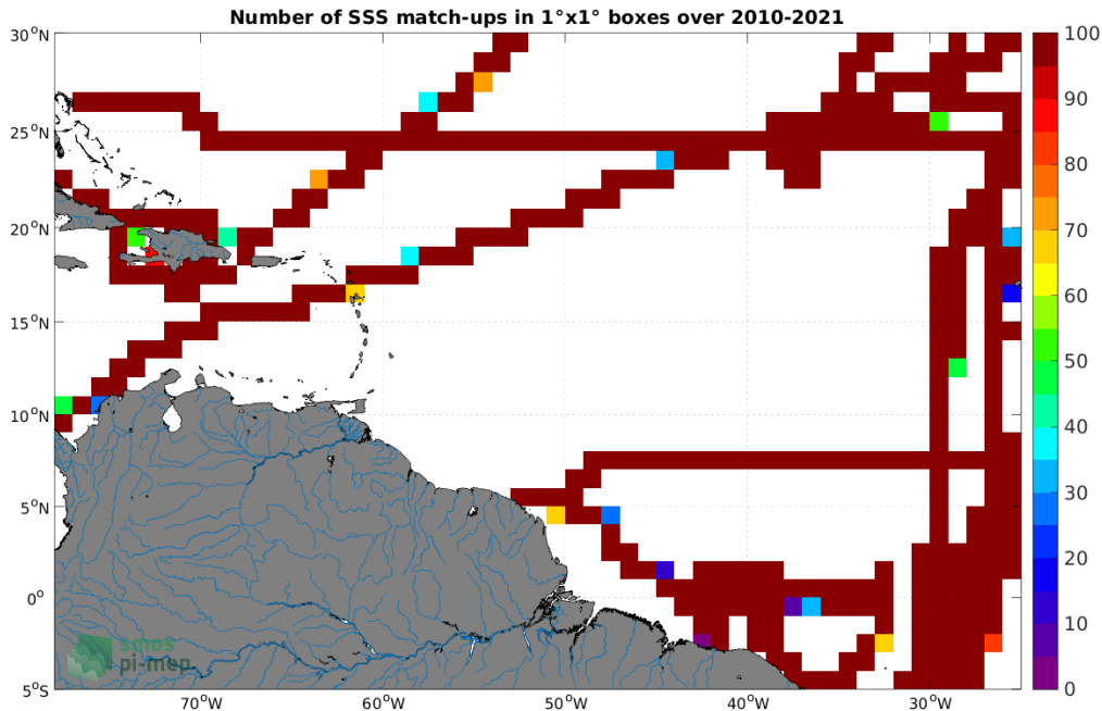
Figure 4: Number of SSS match-ups between TSG (CSIC-UTM) SSS and the SMOS SSS L3 v8 - 18 Days (CATDS-CECOS-LOCEAN) SSS product for the Amazon and Orinoco river plumes Pi-MEP region over 1^\circ \times 1^\circ boxes and for the full satellite product period.
