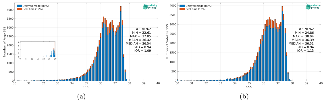
Figure 2: Histograms of SSS from Argo (a) and SMOS SSS L3 v8 - 18 Days (CATDS-CEC-LOCEAN) (b) considering all match-up pairs per bins of 0.1 over the Amazon and Orinoco river plumes Pi-MEP region and for the full satellite product period.
