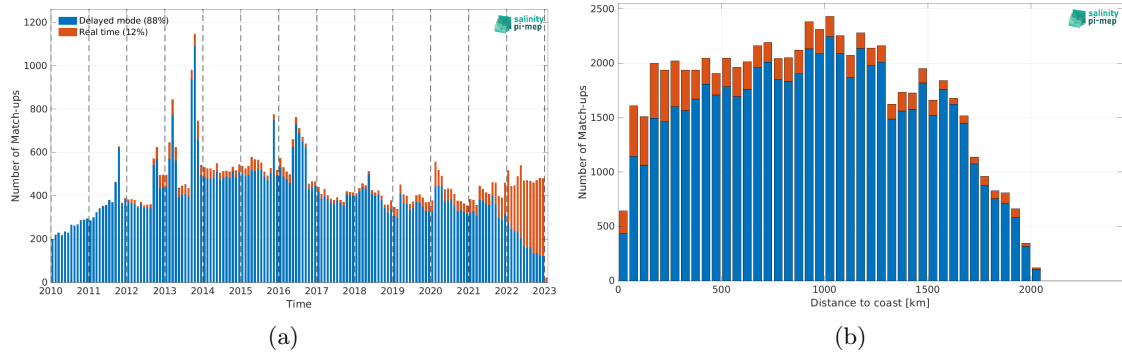
Figure 1: Number of match-ups between Argo and SMOS SSS L3 v8 - 18 Days (CATDS-CEC-LOCEAN) SSS as a function of time (a) and as function of the distance to coast (b) over the Amazon and Orinoco river plumes Pi-MEP region and for the full satellite product period.
