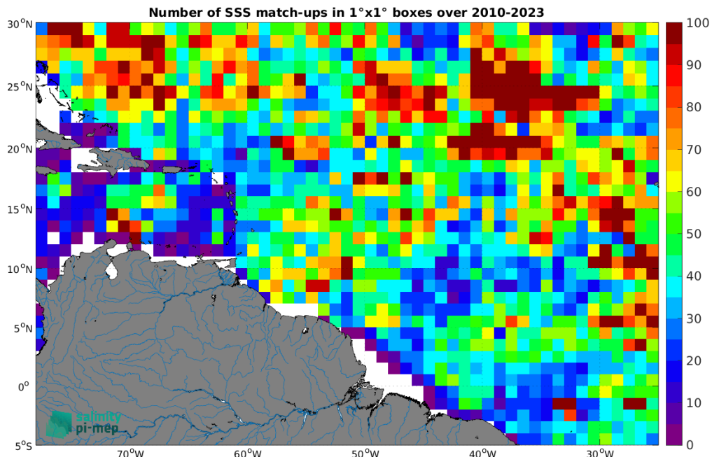
Figure 4: Number of SSS match-ups between Argo SSS and the SMOS SSS L3 v8 - 18 Days (CATDS-CEC-LOCEAN) SSS product for the Amazon and Orinoco river plumes Pi-MEP region over 1^\circ \times 1^\circ boxes and for the full satellite product period.
