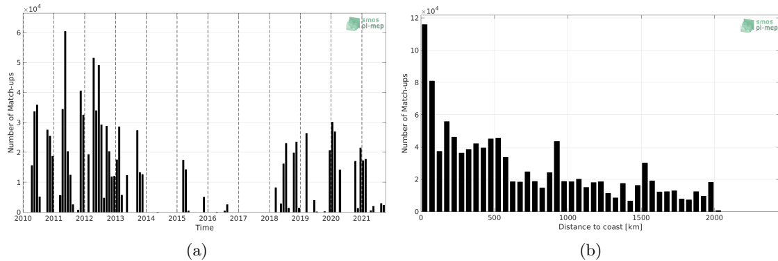
Figure 1: Number of match-ups between TSG (SAMOS) and SMOS SSS L3 v7 - 9 Days (CATDS-CECOS-LOCEAN) SSS as a function of time (a) and as function of the distance to coast (b) over the Amazon and Orinoco river plumes Pi-MEP region and for the full satellite product period.
