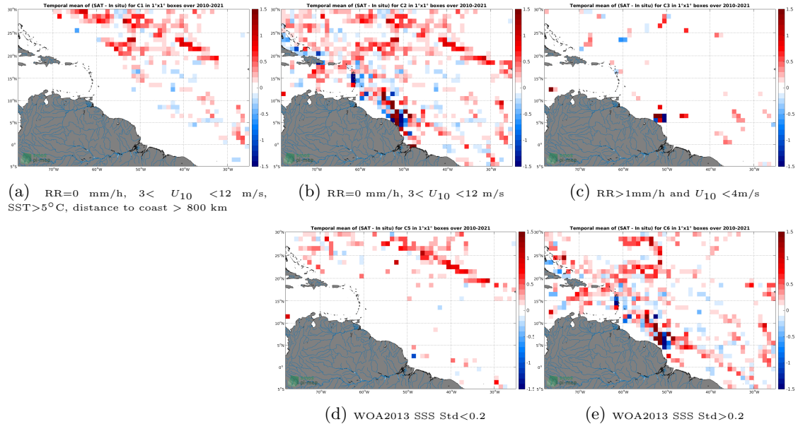
Figure 12: Temporal mean gridded over spatial boxes of size 1^{\circ}\times 1^{\circ} of \Delta\text{SSS} (SMOS SSS L3 v7 - 9 Days (CATDS-CECOS-LOCEAN) - TSG (SAMOS)) for 5 different subdatasets corresponding to:RR=0 mm/h, 3 < U_{10} < 12 m/s, SST >5^{\circ}\text{C} , distance to coast > 800 km (a), RR=0 mm/h, 3 < U_{10} < 12 m/s (b), RR >1 mm/h and U_{10} < 4 m/s (c), WOA2013 SSS Std <0.2 (d), WOA2013 SSS Std >0.2 (e).
