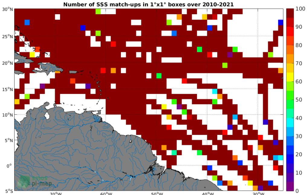
Figure 4: Number of SSS match-ups between TSG (SAMOS) SSS and the SMOS SSS L3 v7 - 9 Days (CATDS-CECOS-LOCEAN) SSS product for the Amazon and Orinoco river plumes Pi-MEP region over 1^{\circ} \times 1^{\circ} boxes and for the full satellite product period.
