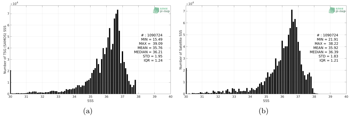
Figure 2: Histograms of SSS from TSG (SAMOS) (a) and SMOS SSS L3 v7 - 9 Days (CATDS-CECOS-LOCEAN) (b) considering all match-up pairs per bins of 0.1 over the Amazon and Orinoco river plumes Pi-MEP region and for the full satellite product period.
