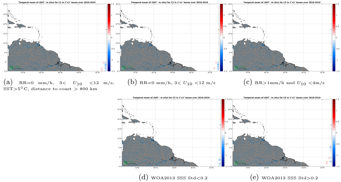
Figure 12: Temporal mean gridded over spatial boxes of size 1^{\circ}\times 1^{\circ} of \Delta\text{SSS} (SMOS SSS L3 v7 - 9 Days (CATDS-CECOS-LOCEAN) - TSG (Polarstern)) for 5 different subdatasets corresponding to:RR=0 mm/h, 3 < U_{10} < 12 m/s, SST >5^{\circ}\text{C} , distance to coast > 800 km (a), RR=0 mm/h, 3 < U_{10} < 12 m/s (b), RR >1 mm/h and U_{10} < 4 m/s (c), WOA2013 SSS Std <0.2 (d), WOA2013 SSS Std >0.2 (e).
