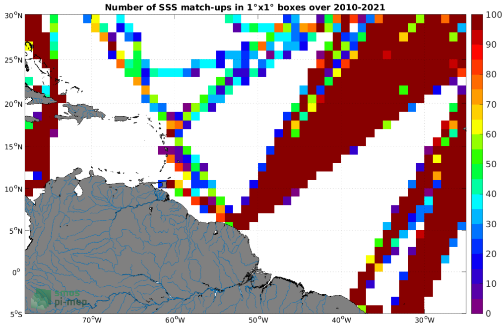
Figure 4: Number of SSS match-ups between TSG (LEGOS-DM) SSS and the SMOS SSS L3 v7 - 9 Days (CATDS-CECOS-LOCEAN) SSS product for the Amazon and Orinoco river plumes Pi-MEP region over 1^\circ \times 1^\circ boxes and for the full satellite product period.
