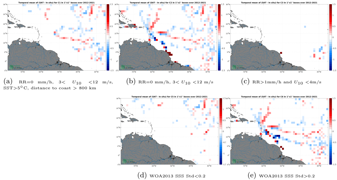
Figure 12: Temporal mean gridded over spatial boxes of size 1^{\circ}\times 1^{\circ} of \Delta SSS (SMOS SSS L3 v7 - 9 Days (CATDS-CECOS-LOCEAN) - TSG (GOSUD-Sailing-ship)) for 5 different subdatasets corresponding to:RR=0 mm/h, 3 < U_{10} < 12 m/s, SST >5^{\circ}\text{C} , distance to coast > 800 km (a), RR=0 mm/h, 3 < U_{10} < 12 m/s (b), RR >1 mm/h and U_{10} < 4 m/s (c), WOA2013 SSS Std <0.2 (d), WOA2013 SSS Std >0.2 (e).
