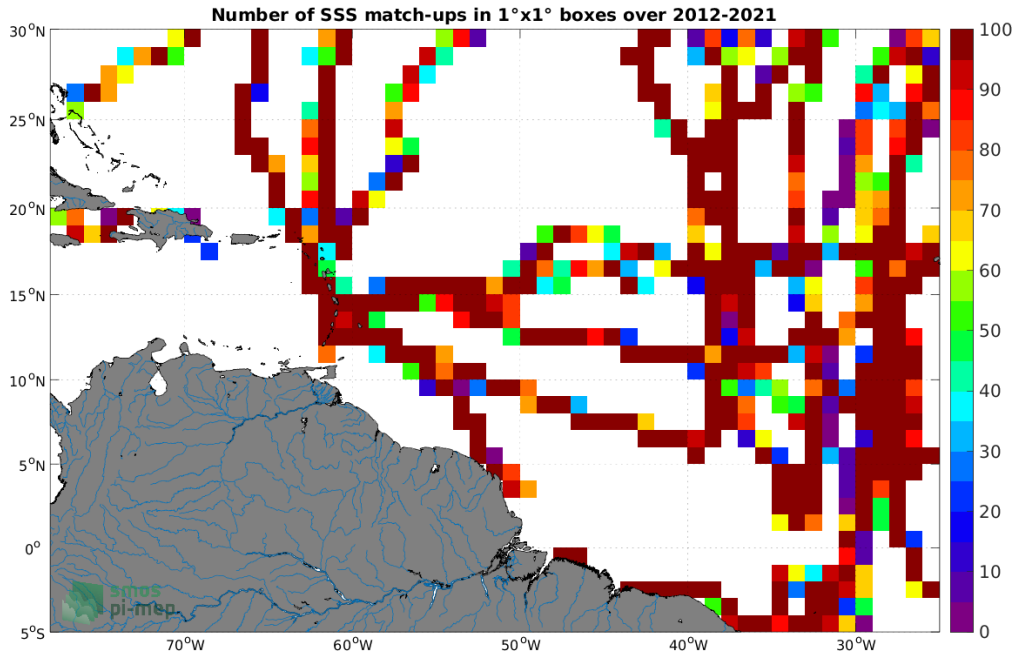
Figure 4: Number of SSS match-ups between TSG (GOSUD-Sailing-ship) SSS and the SMOS SSS L3 v7 - 9 Days (CATDS-CECOS-LOCEAN) SSS product for the Amazon and Orinoco river plumes Pi-MEP region over 1^\circ \times 1^\circ boxes and for the full satellite product period.
