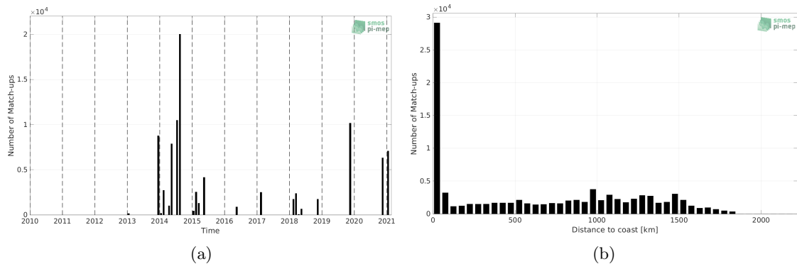
Figure 1: Number of match-ups between TSG (GOSUD-Sailing-ship) and SMOS SSS L3 v7 - 9 Days (CATDS-CECOS-LOCEAN) SSS as a function of time (a) and as function of the distance to coast (b) over the Amazon and Orinoco river plumes Pi-MEP region and for the full satellite product period.
