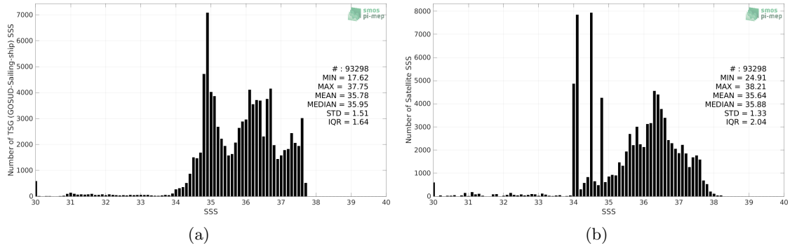
Figure 2: Histograms of SSS from TSG (GOSUD-Sailing-ship) (a) and SMOS SSS L3 v7 - 9 Days (CATDS-CECOS-LOCEAN) (b) considering all match-up pairs per bins of 0.1 over the Amazon and Orinoco river plumes Pi-MEP region and for the full satellite product period.
