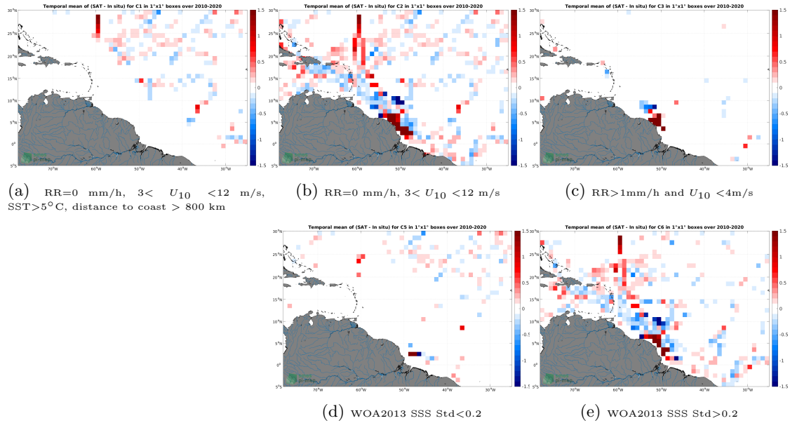
Figure 12: Temporal mean gridded over spatial boxes of size 1^{\circ}\times 1^{\circ} of \Delta SSS (SMOS SSS L3 v7 - 9 Days (CATDS-CECOS-LOCEAN) - TSG (GOSUD-Research-vessel)) for 5 different subdatasets corresponding to:RR=0 mm/h, 3 < U_{10} < 12 m/s, SST >5^{\circ}\text{C} , distance to coast > 800 km (a), RR=0 mm/h, 3 < U_{10} < 12 m/s (b), RR >1 mm/h and U_{10} < 4 m/s (c), WOA2013 SSS Std <0.2 (d), WOA2013 SSS Std >0.2 (e).
