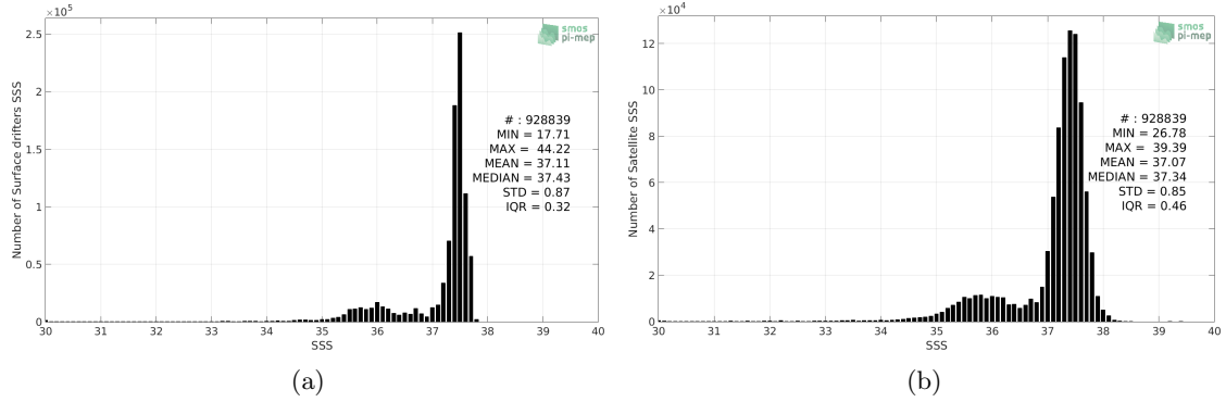
Figure 2: Histograms of SSS from Surface drifters (a) and SMOS SSS L3 v7 - 9 Days (CATDS-CECOS-LOCEAN) (b) considering all match-up pairs per bins of 0.1 over the Amazon and Orinoco river plumes Pi-MEP region and for the full satellite product period.
