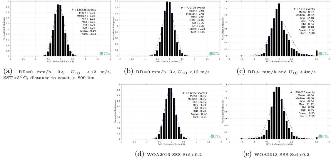
Figure 12: Normalized histogram of \Delta SSS (SMOS SSS L3 v7 - 9 Days (CATDS-CECOS-LOCEAN) - Surface drifters) for 5 different subdatasets corresponding to: RR=0 mm/h, 3 < U_{10} < 12 m/s, SST>5°C, distance to coast > 800 km (a), RR=0 mm/h, 3 < U_{10} < 12 m/s (b), RR>1mm/h and U_{10} < 4 m/s (c), WOA2013 SSS Std<0.2 (d), WOA2013 SSS Std>0.2 (e).
