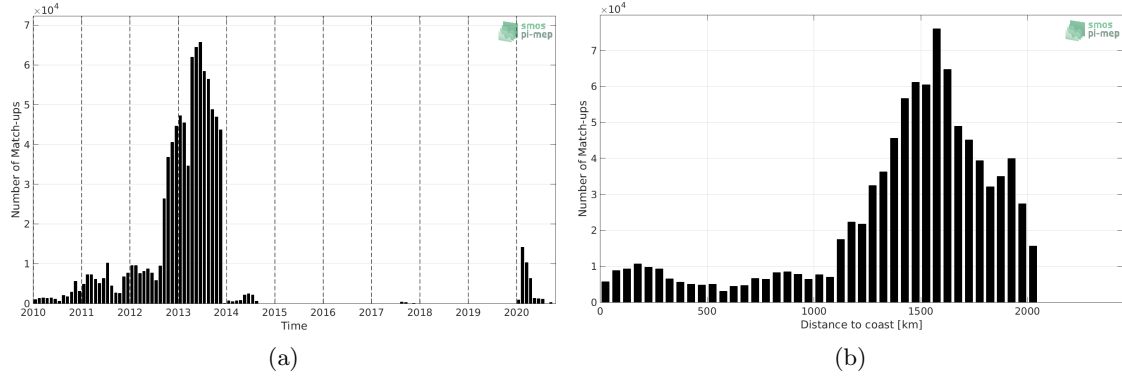
Figure 1: Number of match-ups between Surface drifters and SMOS SSS L3 v7 - 9 Days (CATDS-CECOS-LOCEAN) SSS as a function of time (a) and as function of the distance to coast (b) over the Amazon and Orinoco river plumes Pi-MEP region and for the full satellite product period.
