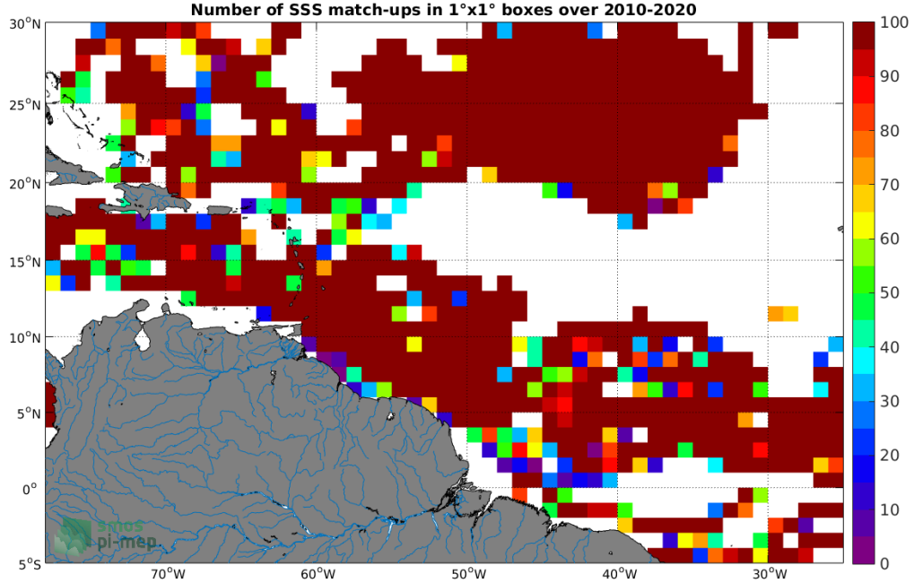
Figure 3: Number of SSS match-ups between Surface drifters SSS and the SMOS SSS L3 v7 - 9 Days (CATDS-CECOS-LOCEAN) SSS product for the Amazon and Orinoco river plumes Pi-MEP region over 1^\circ \times 1^\circ boxes and for the full satellite product period.
