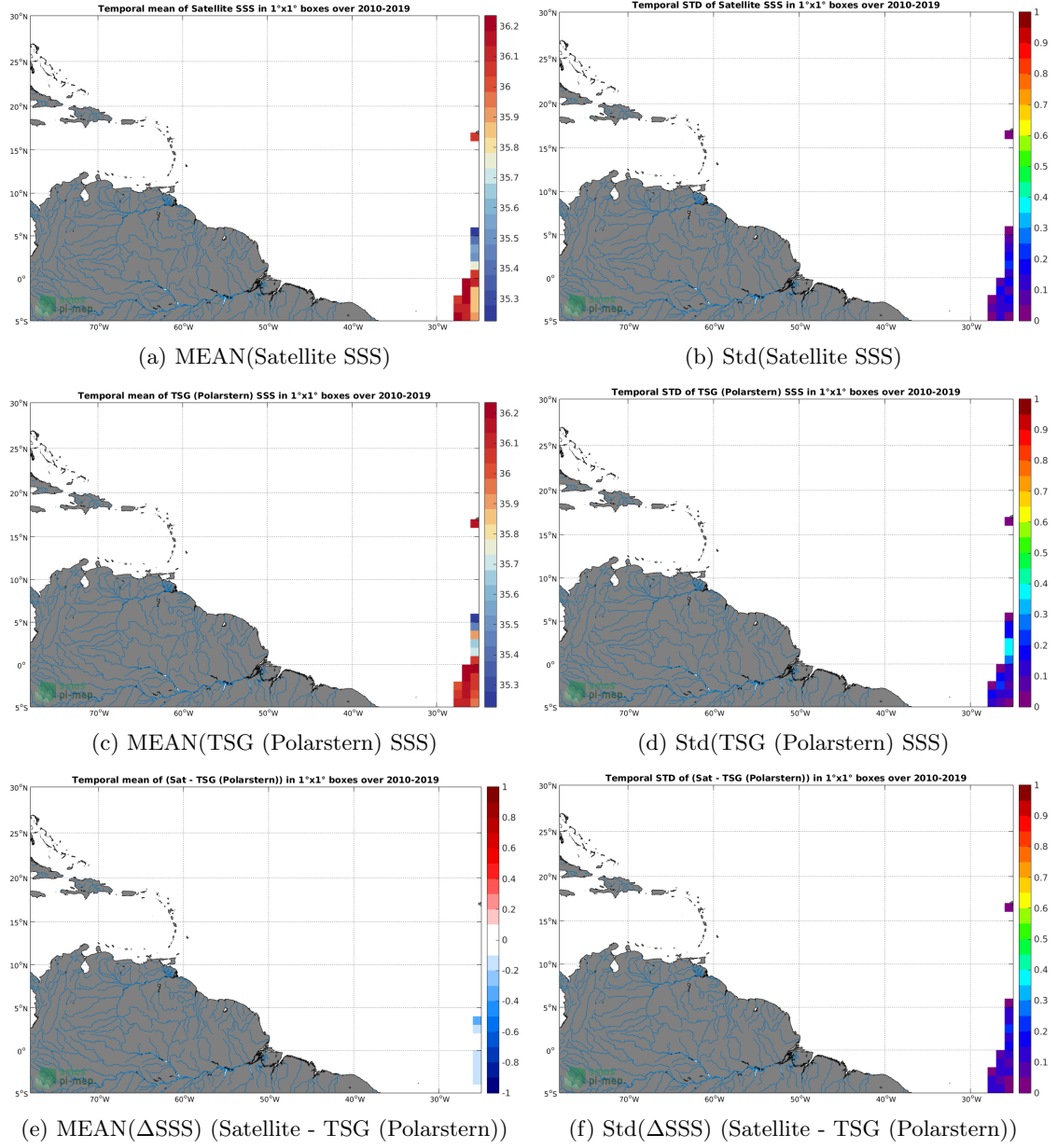
Figure 6: Temporal mean (left) and Std (right) of SSS from SMOS SSS L3 v7 - 18 Days (CATDS-CECOS-LOCEAN) (top), TSG (Polarstern) (middle), and of \Delta SSS (Satellite - TSG (Polarstern)). Only match-up pairs are used to generate these maps.
