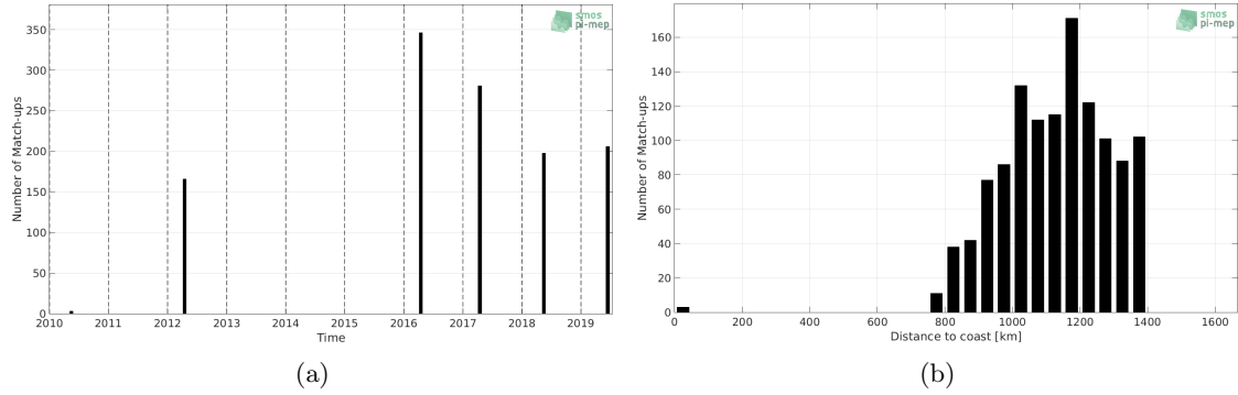
Figure 1: Number of match-ups between TSG (Polarstern) and SMOS SSS L3 v7 - 18 Days (CATDS-CECOS-LOCEAN) SSS as a function of time (a) and as function of the distance to coast (b) over the Amazon and Orinoco river plumes Pi-MEP region and for the full satellite product period.
