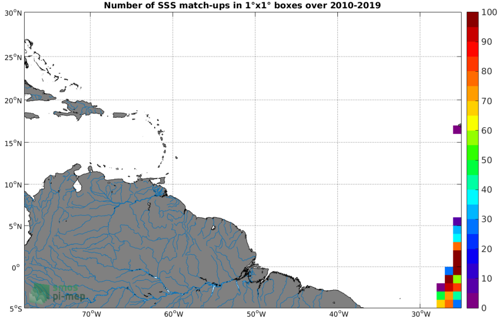
Figure 4: Number of SSS match-ups between TSG (Polarstern) SSS and the SMOS SSS L3 v7 - 18 Days (CATDS-CECOS-LOCEAN) SSS product for the Amazon and Orinoco river plumes Pi-MEP region over 1^\circ \times 1^\circ boxes and for the full satellite product period.
