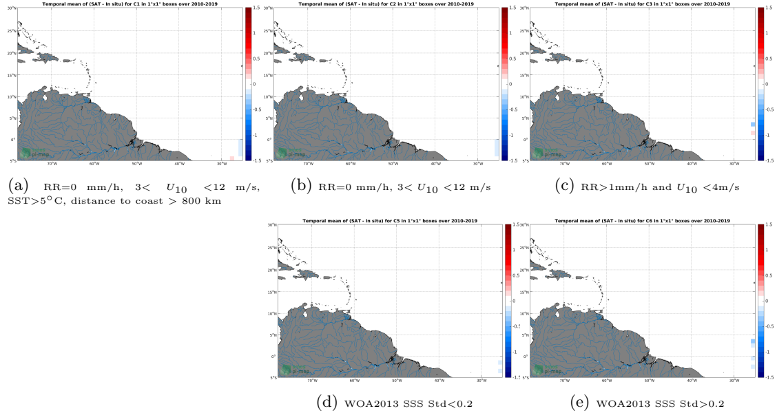
Figure 12: Temporal mean gridded over spatial boxes of size 1^{\circ}\times 1^{\circ} of \Delta\text{SSS} (SMOS SSS L3 v7 - 18 Days (CATDS-CECOS-LOCEAN) - TSG (Polarstern)) for 5 different subdatasets corresponding to: RR=0 mm/h, 3 < U_{10} < 12 m/s, SST >5^{\circ}\text{C} , distance to coast > 800 km (a), RR=0 mm/h, 3 < U_{10} < 12 m/s (b), RR >1 mm/h and U_{10} < 4 m/s (c), WOA2013 SSS Std <0.2 (d), WOA2013 SSS Std >0.2 (e).
