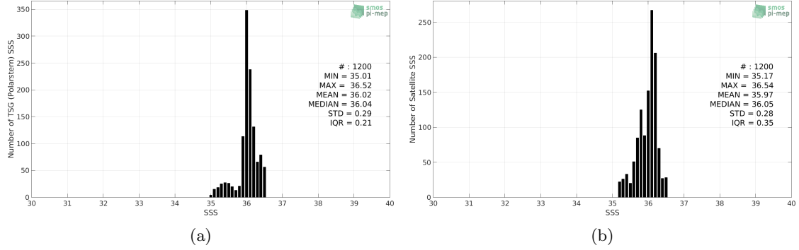
Figure 2: Histograms of SSS from TSG (Polarstern) (a) and SMOS SSS L3 v7 - 18 Days (CATDS-CECOS-LOCEAN) (b) considering all match-up pairs per bins of 0.1 over the Amazon and Orinoco river plumes Pi-MEP region and for the full satellite product period.
