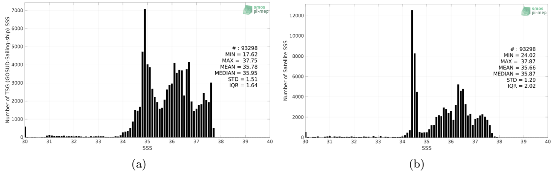
Figure 2: Histograms of SSS from TSG (GOSUD-Sailing-ship) (a) and SMOS SSS L3 v7 - 18 Days (CATDS-CECOS-LOCEAN) (b) considering all match-up pairs per bins of 0.1 over the Amazon and Orinoco river plumes Pi-MEP region and for the full satellite product period.
