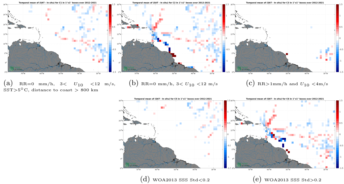
Figure 12: Temporal mean gridded over spatial boxes of size 1^{\circ}\times 1^{\circ} of \Delta SSS (SMOS SSS L3 v7 - 18 Days (CATDS-CECOS-LOCEAN) - TSG (GOSUD-Sailing-ship)) for 5 different subdatasets corresponding to:RR=0 mm/h, 3 < U_{10} < 12 m/s, SST > 5^{\circ}\text{C} , distance to coast > 800 km (a), RR=0 mm/h, 3 < U_{10} < 12 m/s (b), RR > 1 mm/h and U_{10} < 4 m/s (c), WOA2013 SSS Std < 0.2 (d), WOA2013 SSS Std > 0.2 (e).
