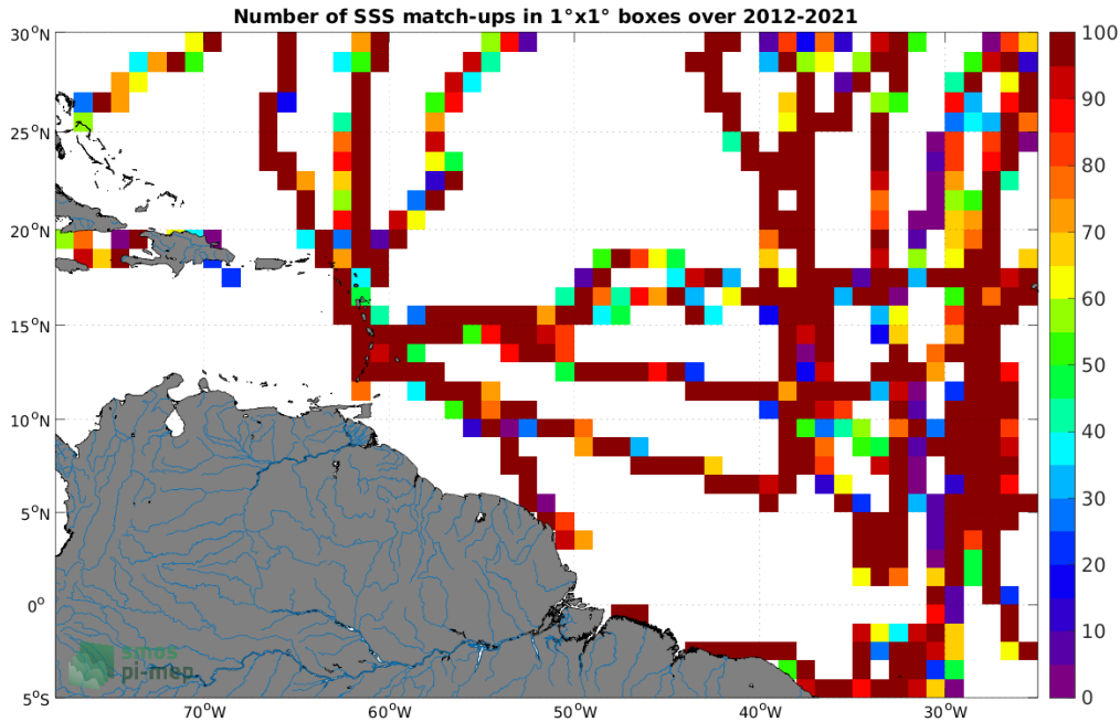
Figure 4: Number of SSS match-ups between TSG (GOSUD-Sailing-ship) SSS and the SMOS SSS L3 v7 - 18 Days (CATDS-CECOS-LOCEAN) SSS product for the Amazon and Orinoco river plumes Pi-MEP region over 1^{\circ} \times 1^{\circ} boxes and for the full satellite product period.
