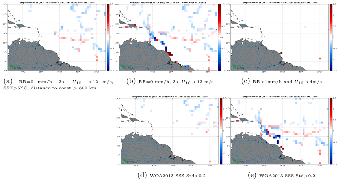
Figure 12: Temporal mean gridded over spatial boxes of size 1^{\circ}\times 1^{\circ} of \Delta SSS (SMOS SSS L3 v7 - 18 Days (CATDS-CECOS-LOCEAN) - TSG (GOSUD-Sailing-ship)) for 5 different subdatasets corresponding to:RR=0 mm/h, 3 < U_{10} < 12 m/s, SST >5^{\circ}\text{C} , distance to coast > 800 km (a), RR=0 mm/h, 3 < U_{10} < 12 m/s (b), RR >1 mm/h and U_{10} < 4 m/s (c), WOA2013 SSS Std <0.2 (d), WOA2013 SSS Std >0.2 (e).
