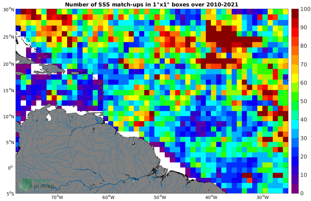
Figure 4: Number of SSS match-ups between Argo SSS and the SMOS SSS L3 v7 - 18 Days (CATDS-CECOS-LOCEAN) SSS product for the Amazon and Orinoco river plumes Pi-MEP region over 1^{\circ} \times 1^{\circ} boxes and for the full satellite product period.
