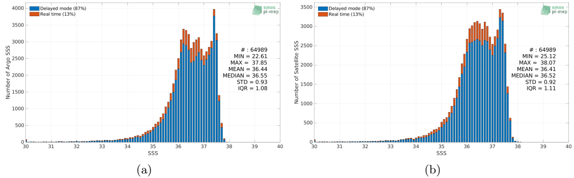
Figure 2: Histograms of SSS from Argo (a) and SMOS SSS L3 v7 - 18 Days (CATDS-CECOS-LOCEAN) (b) considering all match-up pairs per bins of 0.1 over the Amazon and Orinoco river plumes Pi-MEP region and for the full satellite product period.
