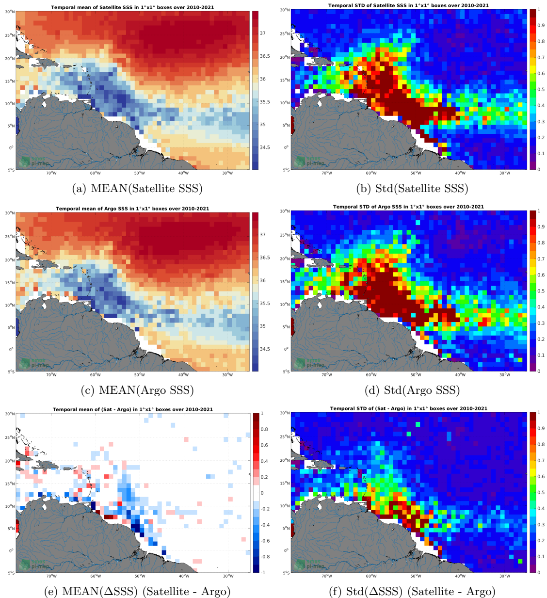
Figure 6: Temporal mean (left) and Std (right) of SSS from SMOS SSS L3 v7 - 18 Days (CATDS-CECOS-LOCEAN) (top), Argo (middle), and of \Delta SSS (Satellite - Argo). Only match-up pairs are used to generate these maps.
