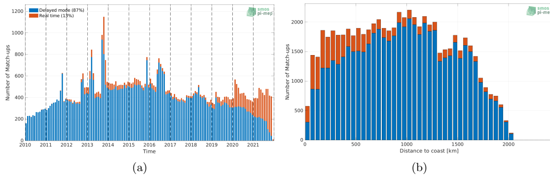
Figure 1: Number of match-ups between Argo and SMOS SSS L3 v7 - 18 Days (CATDS-CECOS-LOCEAN) SSS as a function of time (a) and as function of the distance to coast (b) over the Amazon and Orinoco river plumes Pi-MEP region and for the full satellite product period.
