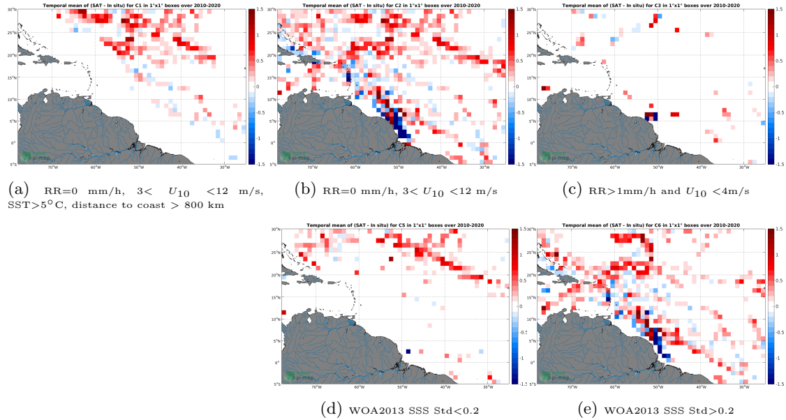
Figure 12: Temporal mean gridded over spatial boxes of size 1^{\circ}\times 1^{\circ} of \Delta\text{SSS} (SMOS SSS L3 v5 - 9 Days (CATDS-CECOS-LOCEAN) - TSG (SAMOS)) for 5 different subdatasets corresponding to:RR=0 mm/h, 3 < U_{10} < 12 m/s, SST >5^{\circ}\text{C} , distance to coast > 800 km (a), RR=0 mm/h, 3 < U_{10} < 12 m/s (b), RR >1 mm/h and U_{10} < 4 m/s (c), WOA2013 SSS Std <0.2 (d), WOA2013 SSS Std >0.2 (e).
