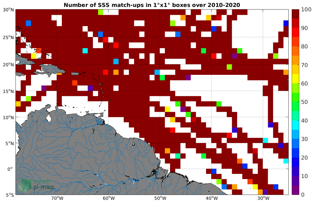
Figure 4: Number of SSS match-ups between TSG (SAMOS) SSS and the SMOS SSS L3 v5 - 9 Days (CATDS-CECOS-LOCEAN) SSS product for the Amazon and Orinoco river plumes Pi-MEP region over 1°x1° boxes and for the full satellite product period.
