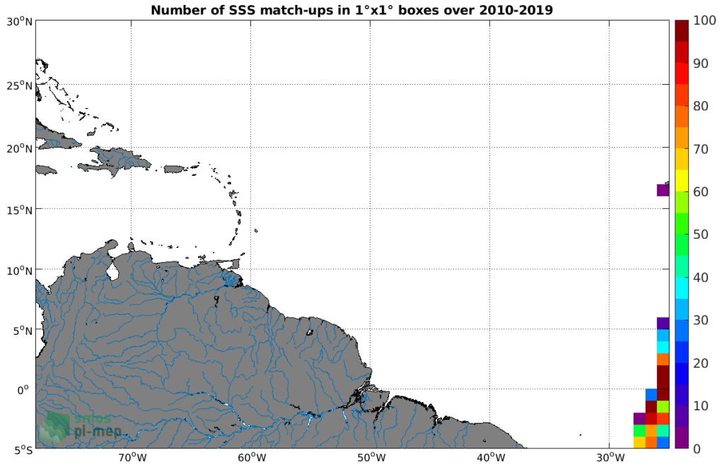
Figure 4: Number of SSS match-ups between TSG (Polarstern) SSS and the SMOS SSS L3 v5 - 9 Days (CATDS-CECOS-LOCEAN) SSS product for the Amazon and Orinoco river plumes Pi-MEP region over 1°×1° boxes and for the full satellite product period.
