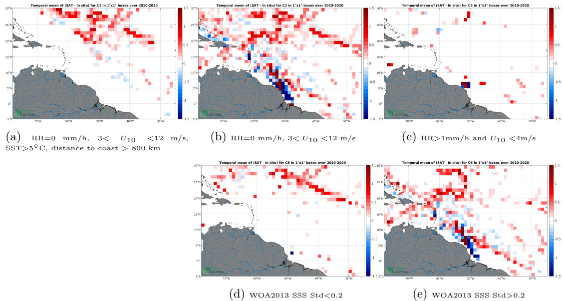
Figure 12: Temporal mean gridded over spatial boxes of size 1^{\circ}\times 1^{\circ} of \Delta\text{SSS} (SMOS SSS L3 v5 - 18 Days (CATDS-CECOS-LOCEAN) - TSG (SAMOS)) for 5 different subdatasets corresponding to:RR=0 mm/h, 3 < U_{10} < 12 m/s, SST >5^{\circ}\text{C} , distance to coast > 800 km (a), RR=0 mm/h, 3 < U_{10} < 12 m/s (b), RR >1 mm/h and U_{10} < 4 m/s (c), WOA2013 SSS Std <0.2 (d), WOA2013 SSS Std >0.2 (e).
