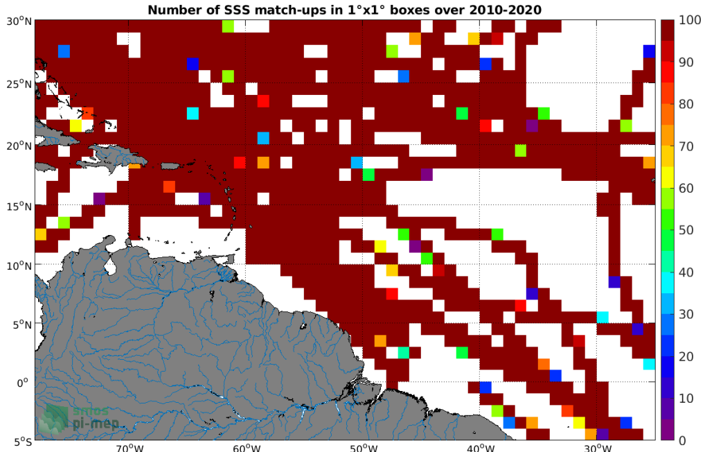
Figure 4: Number of SSS match-ups between TSG (SAMOS) SSS and the SMOS SSS L3 v5 - 18 Days (CATDS-CECOS-LOCEAN) SSS product for the Amazon and Orinoco river plumes Pi-MEP region over 1^{\circ} \times 1^{\circ} boxes and for the full satellite product period.
