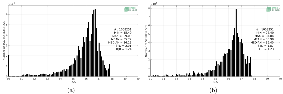
Figure 2: Histograms of SSS from TSG (SAMOS) (a) and SMOS SSS L3 v5 - 18 Days (CATDS-CECOS-LOCEAN) (b) considering all match-up pairs per bins of 0.1 over the Amazon and Orinoco river plumes Pi-MEP region and for the full satellite product period.
