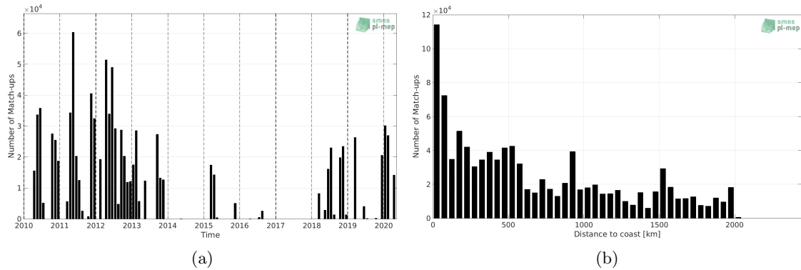
Figure 1: Number of match-ups between TSG (SAMOS) and SMOS SSS L3 v5 - 18 Days (CATDS-CECOS-LOCEAN) SSS as a function of time (a) and as function of the distance to coast (b) over the Amazon and Orinoco river plumes Pi-MEP region and for the full satellite product period.
