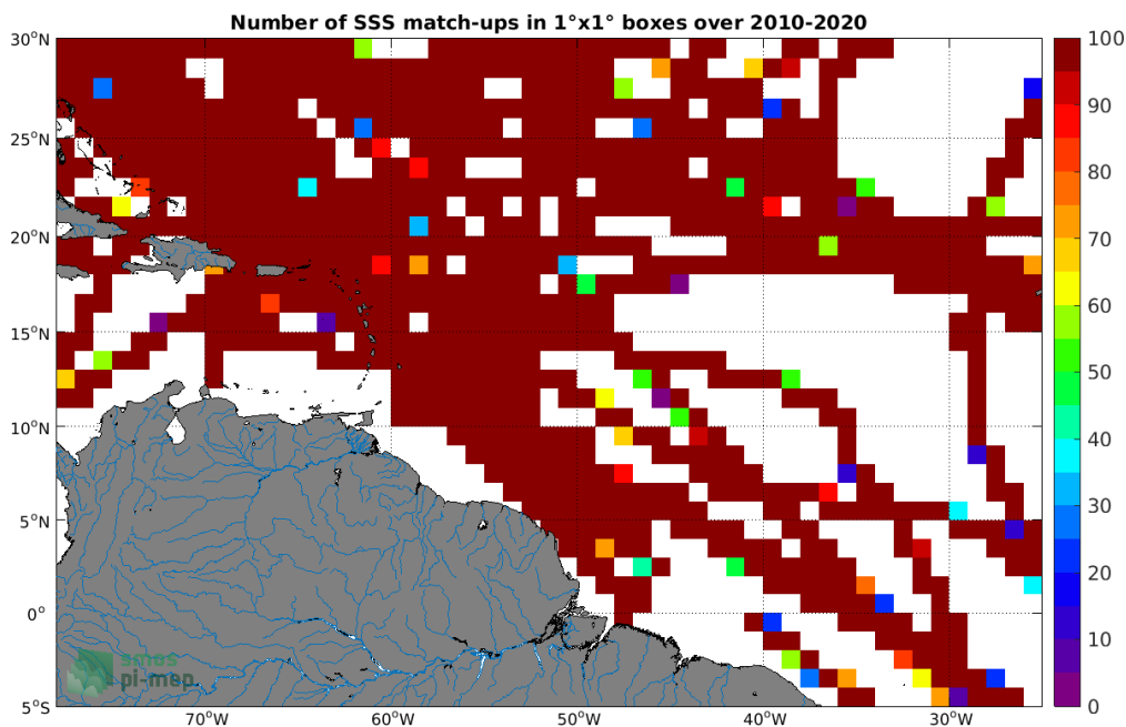
Figure 4: Number of SSS match-ups between TSG (SAMOS) SSS and the SMOS SSS L3 v5 - 18 Days (CATDS-CECOS-LOCEAN) SSS product for the Amazon and Orinoco river plumes Pi-MEP region over 1^\circ \times 1^\circ boxes and for the full satellite product period.
