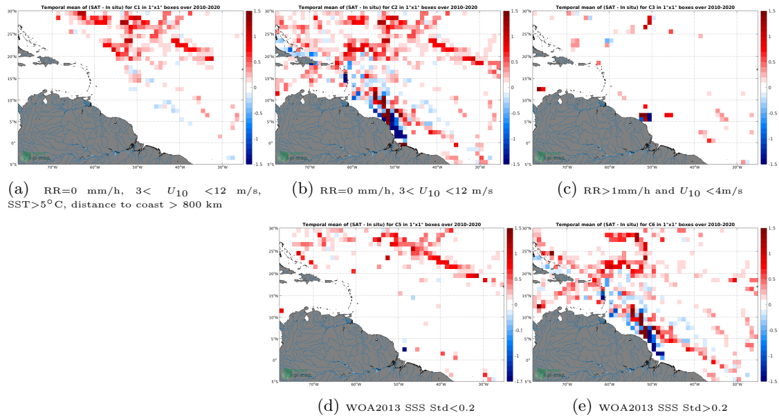
Figure 12: Temporal mean gridded over spatial boxes of size 1^{\circ}\times 1^{\circ} of \Delta\text{SSS} (SMOS SSS L3 v5 - 18 Days (CATDS-CECOS-LOCEAN) - TSG (SAMOS)) for 5 different subdatasets corresponding to:RR=0 mm/h, 3 < U_{10} < 12 m/s, SST >5^{\circ}\text{C} , distance to coast > 800 km (a), RR=0 mm/h, 3 < U_{10} < 12 m/s (b), RR >1 mm/h and U_{10} < 4 m/s (c), WOA2013 SSS Std <0.2 (d), WOA2013 SSS Std >0.2 (e).
