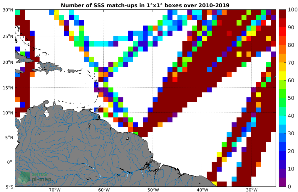
Figure 4: Number of SSS match-ups between TSG (LEGOS-DM) SSS and the SMOS SSS L3 v5 - 18 Days (CATDS-CECOS-LOCEAN) SSS product for the Amazon and Orinoco river plumes Pi-MEP region over 1°x1° boxes and for the full satellite product period.
