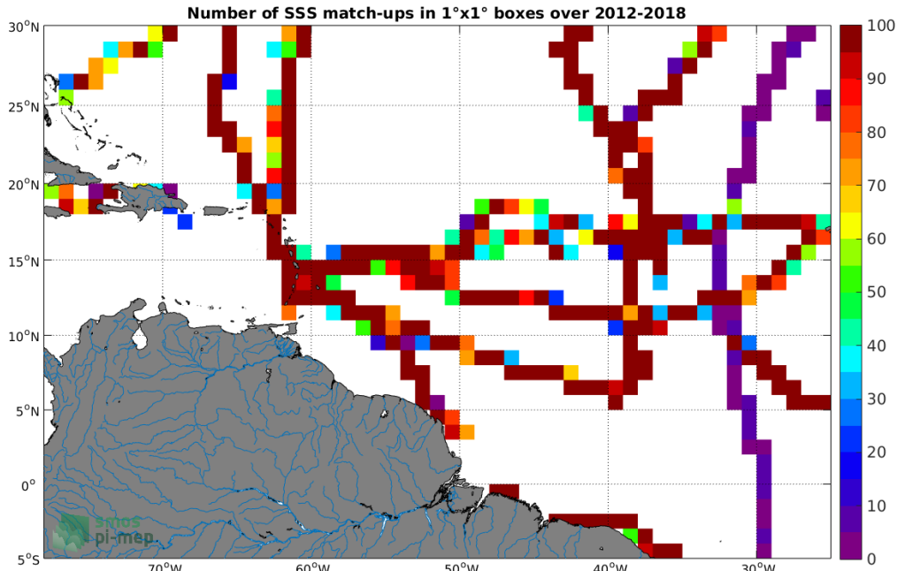
Figure 4: Number of SSS match-ups between TSG (GOSUD-Sailing-ship) SSS and the SMOS SSS L3 v5 - 18 Days (CATDS-CECOS-LOCEAN) SSS product for the Amazon and Orinoco river plumes Pi-MEP region over 1°x1° boxes and for the full satellite product period.
