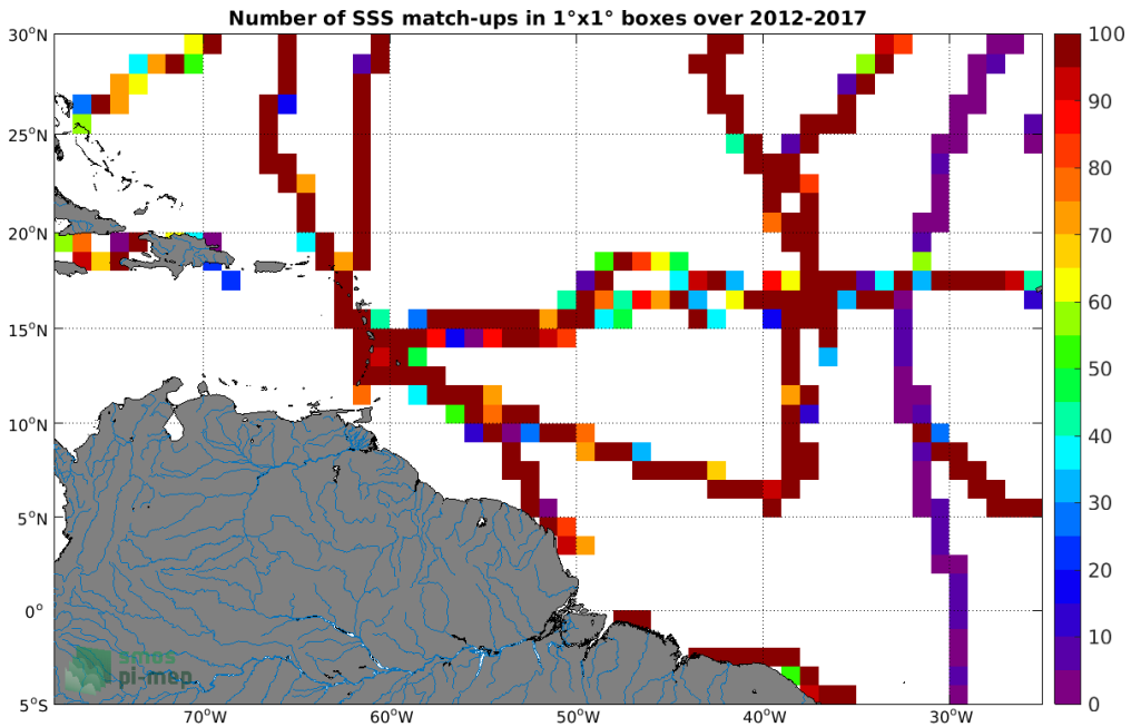
Figure 4: Number of SSS match-ups between TSG (GOSUD-Sailing-ship) SSS and the SMOS SSS L3 v5 - 18 Days (CATDS-CECOS-LOCEAN) SSS product for the Amazon and Orinoco river plumes Pi-MEP region over 1^\circ \times 1^\circ boxes and for the full satellite product period.
