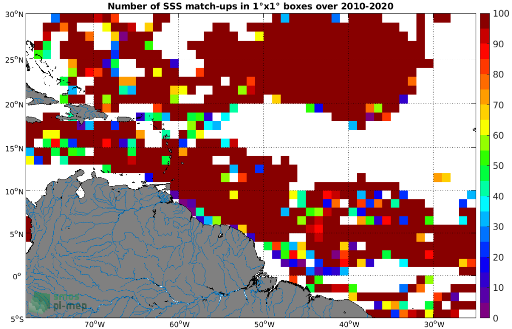
Figure 3: Number of SSS match-ups between Surface drifters SSS and the SMOS SSS L3 v5 - 18 Days (CATDS-CECOS-LOCEAN) SSS product for the Amazon and Orinoco river plumes Pi-MEP region over 1^\circ \times 1^\circ boxes and for the full satellite product period.
