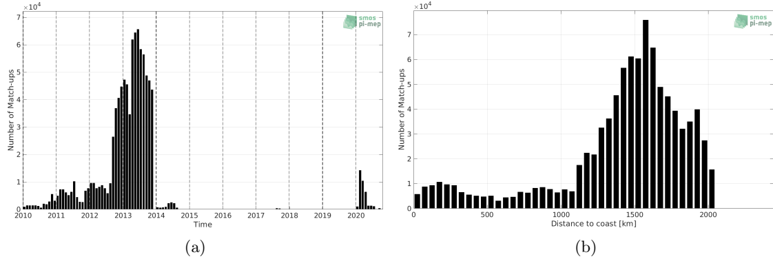
Figure 1: Number of match-ups between Surface drifters and SMOS SSS L3 v5 - 18 Days (CATDS-CECOS-LOCEAN) SSS as a function of time (a) and as function of the distance to coast (b) over the Amazon and Orinoco river plumes Pi-MEP region and for the full satellite product period.
