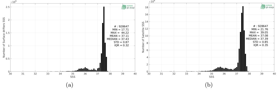
Figure 2: Histograms of SSS from Surface drifters (a) and SMOS SSS L3 v5 - 18 Days (CATDS-CECOS-LOCEAN) (b) considering all match-up pairs per bins of 0.1 over the Amazon and Orinoco river plumes Pi-MEP region and for the full satellite product period.
