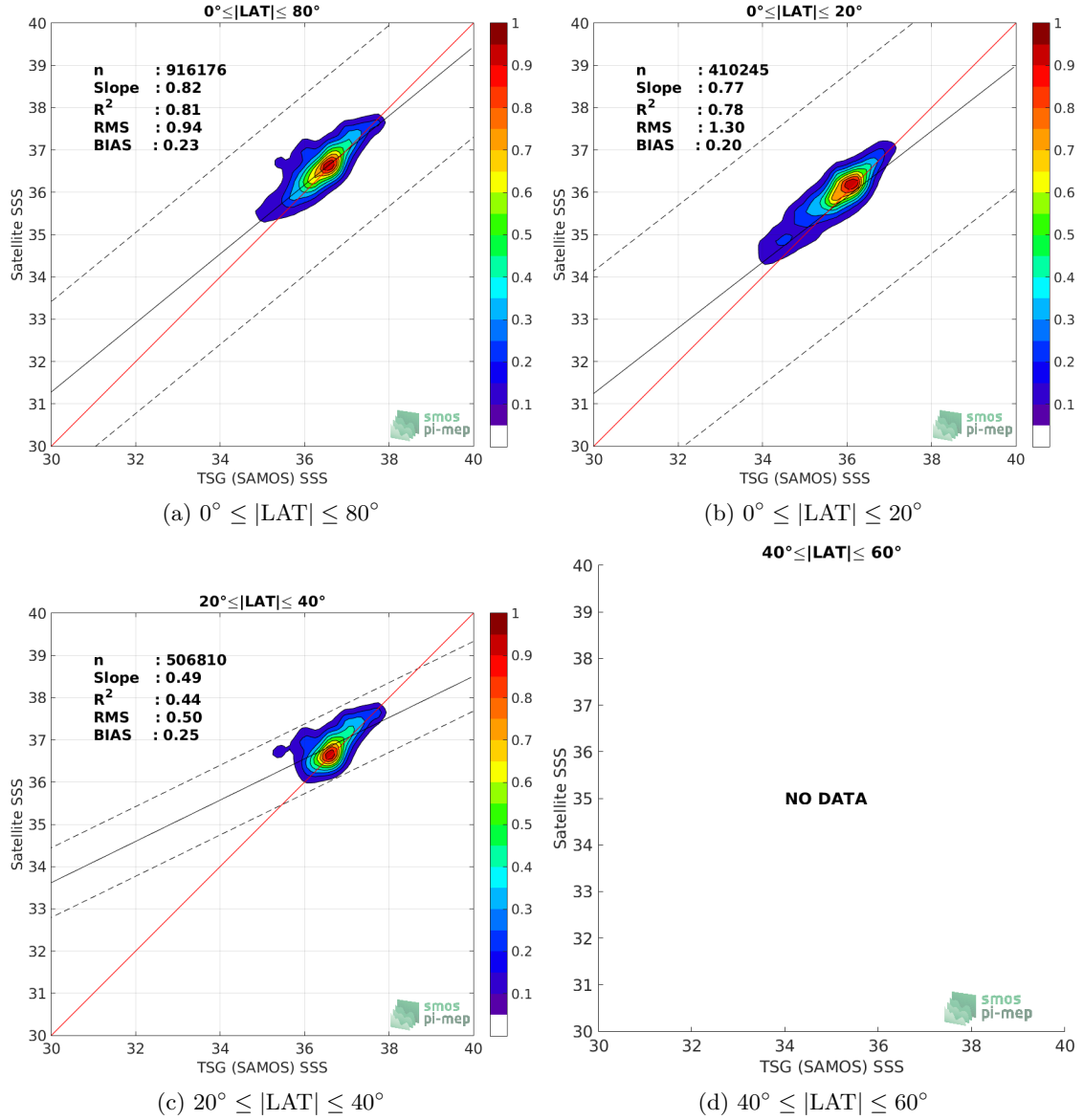
Figure 9: Contour maps of the concentration of SMOS SSS L3 v4 - 18 Days (CATDS-CECOS-LOCEAN) SSS (y-axis) versus TSG (SAMOS) SSS (x-axis) at match-up pairs for different latitude bands. For each plot, the red line shows x=y . The black thin and dashed lines indicate a linear fit through the data cloud and the \pm 95\% confidence levels, respectively. The number match-up pairs n , the slope and R^2 coefficient of the linear fit, the root mean square (RMS) and the mean bias between satellite and in situ data are indicated for each latitude band in each plots.
