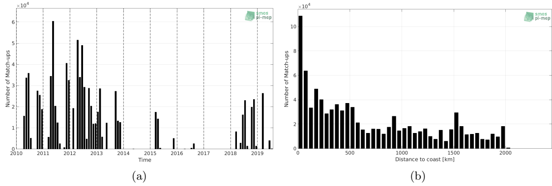
Figure 1: Number of match-ups between TSG (SAMOS) and SMOS SSS L3 v4 - 18 Days (CATDS-CECOS-LOCEAN) SSS as a function of time (a) and as function of the distance to coast (b) over the Amazon and Orinoco river plumes Pi-MEP region and for the full satellite product period.
