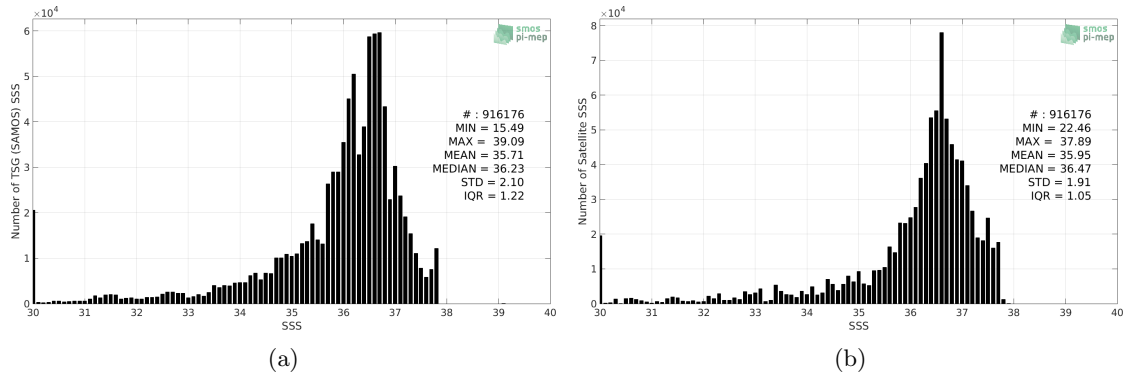
Figure 2: Histograms of SSS from TSG (SAMOS) (a) and SMOS SSS L3 v4 - 18 Days (CATDS-CECOS-LOCEAN) (b) considering all match-up pairs per bins of 0.1 over the Amazon and Orinoco river plumes Pi-MEP region and for the full satellite product period.
