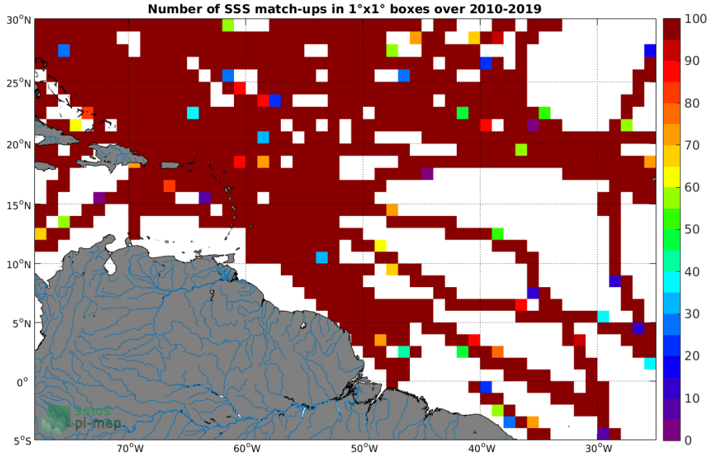
Figure 4: Number of SSS match-ups between TSG (SAMOS) SSS and the SMOS SSS L3 v4 - 18 Days (CATDS-CECOS-LOCEAN) SSS product for the Amazon and Orinoco river plumes Pi-MEP region over 1°x1° boxes and for the full satellite product period.
