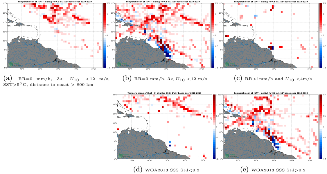
Figure 12: Temporal mean gridded over spatial boxes of size 1^{\circ}\times 1^{\circ} of \Delta\text{SSS} (SMOS SSS L3 v4 - 18 Days (CATDS-CECOS-LOCEAN) - TSG (SAMOS)) for 5 different subdatasets corresponding to: RR=0 mm/h, 3 < U_{10} < 12 m/s, SST > 5^{\circ}\text{C} , distance to coast > 800 km (a), RR=0 mm/h, 3 < U_{10} < 12 m/s (b), RR > 1 mm/h and U_{10} < 4 m/s (c), WOA2013 SSS Std < 0.2 (d), WOA2013 SSS Std > 0.2 (e).
