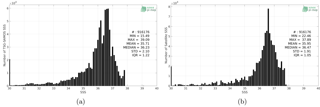
Figure 2: Histograms of SSS from TSG-SAMOS (a) and SMOS-L3-CATDS-CECOS-LOCEAN-V4-18DAYS-25KM (b) considering all match-up pairs per bins of 0.1 over the Amazon and Orinoco river plumes Pi-MEP region and for the full satellite product period.
