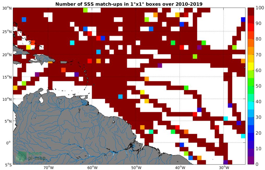
Figure 4: Number of SSS match-ups between TSG-SAMOS SSS and the SMOS-L3-CATDS-CECOS-LOCEAN-V4-18DAYS-25KM SSS product for the Amazon and Orinoco river plumes Pi-MEP region over 1^\circ \times 1^\circ boxes and for the full satellite product period.
