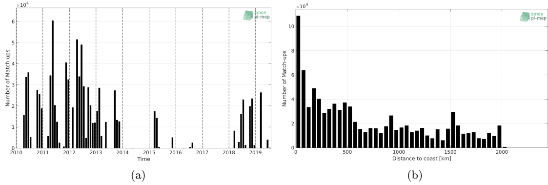
Figure 1: Number of match-ups between TSG-SAMOS and SMOS-L3-CATDS-CECOS-LOCEAN-V4-18DAYS-25KM SSS as a function of time (a) and as function of the distance to coast (b) over the Amazon and Orinoco river plumes Pi-MEP region and for the full satellite product period.
