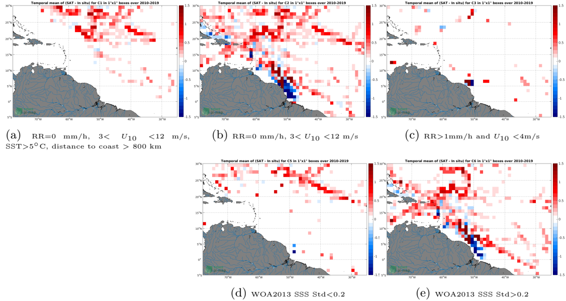
Figure 12: Temporal mean gridded over spatial boxes of size 1^{\circ}\times 1^{\circ} of \Delta\text{SSS} (SMOS-L3-CATDS-CECOS-LOCEAN-V4-18DAYS-25KM - TSG-SAMOS) for 5 different subdatasets corresponding to: \text{RR}=0 mm/h, 3 < U_{10} < 12 m/s, \text{SST} > 5^{\circ}\text{C} , distance to coast > 800 km (a), \text{RR}=0 mm/h, 3 < U_{10} < 12 m/s (b), \text{RR} > 1 mm/h and U_{10} < 4 m/s (c), WOA2013 SSS Std < 0.2 (d), WOA2013 SSS Std > 0.2 (e).
