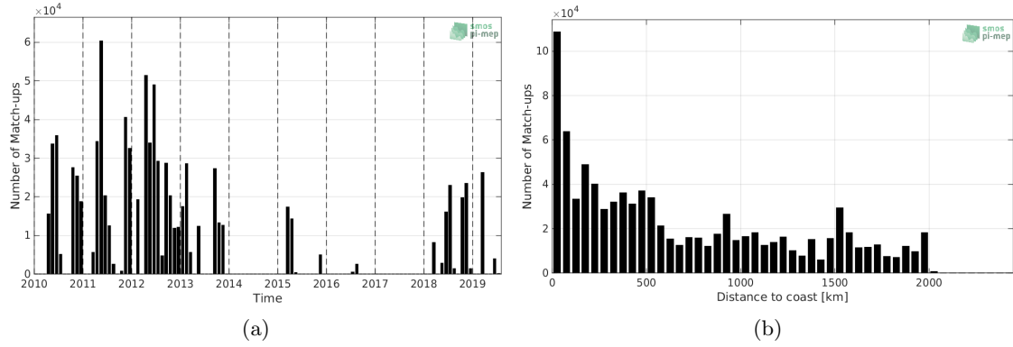
Figure 1: Number of match-ups between TSG-SAMOS and SMOS-L3-CATDS-CECOS-LOCEAN-V4-18DAYS-25KM SSS as a function of time (a) and as function of the distance to coast (b) over the Amazon and Orinoco river plumes Pi-MEP region and for the full satellite product period.
