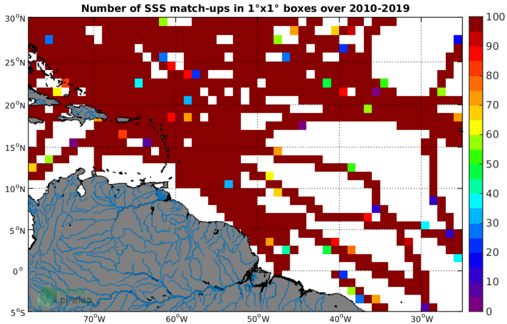
Figure 4: Number of SSS match-ups between TSG-SAMOS SSS and the SMOS-L3-CATDS-CECOS-LOCEAN-V4-18DAYS-25KM SSS product for the Amazon and Orinoco river plumes Pi-MEP region over 1°x1° boxes and for the full satellite product period.
