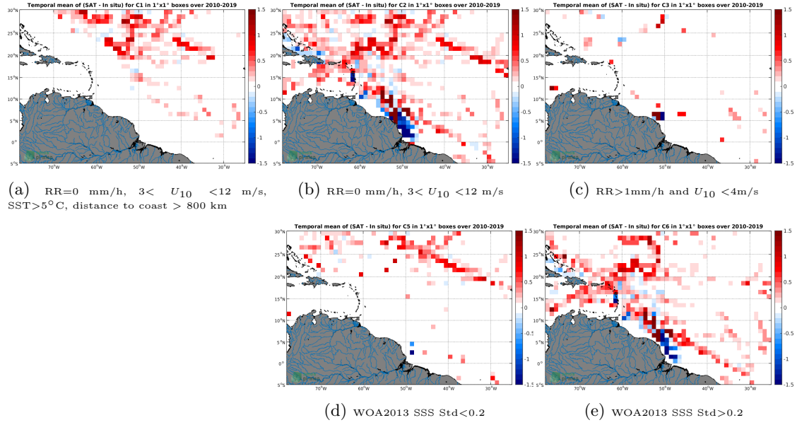
Figure 12: Temporal mean gridded over spatial boxes of size 1^\circ \times 1^\circ of \Delta SSS (SMOS-L3-CATDS-CECOS-LOCEAN-V4-18DAYS-25KM - TSG-SAMOS) for 5 different subdatasets corresponding to: RR=0 mm/h, 3 < U_{10} < 12 m/s, SST > 5^\circ\text{C} , distance to coast > 800 km (a), RR=0 mm/h, 3 < U_{10} < 12 m/s (b), RR > 1 mm/h and U_{10} < 4 m/s (c), WOA2013 SSS Std < 0.2 (d), WOA2013 SSS Std > 0.2 (e).
