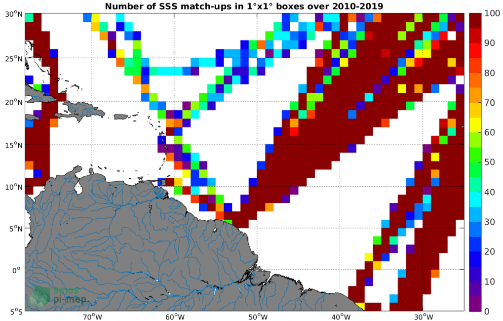
Figure 4: Number of SSS match-ups between TSG (LEGOS-DM) SSS and the SMOS SSS L3 v4 - 18 Days (CATDS-CECOS-LOCEAN) SSS product for the Amazon and Orinoco river plumes Pi-MEP region over 1°x1° boxes and for the full satellite product period.
