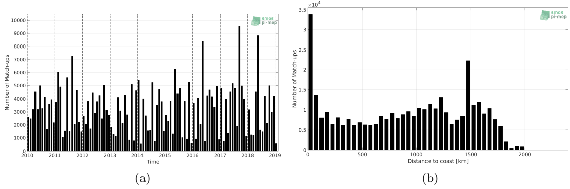
Figure 1: Number of match-ups between TSG (LEGOS-DM) and SMOS SSS L3 v4 - 18 Days (CATDS-CECOS-LOCEAN) SSS as a function of time (a) and as function of the distance to coast (b) over the Amazon and Orinoco river plumes Pi-MEP region and for the full satellite product period.
