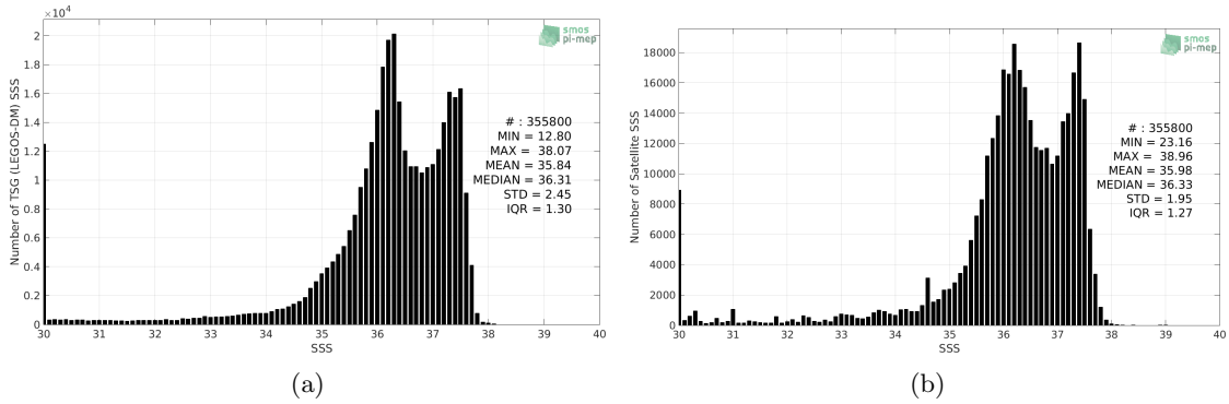
Figure 2: Histograms of SSS from TSG (LEGOS-DM) (a) and SMOS SSS L3 v4 - 18 Days (CATDS-CECOS-LOCEAN) (b) considering all match-up pairs per bins of 0.1 over the Amazon and Orinoco river plumes Pi-MEP region and for the full satellite product period.
