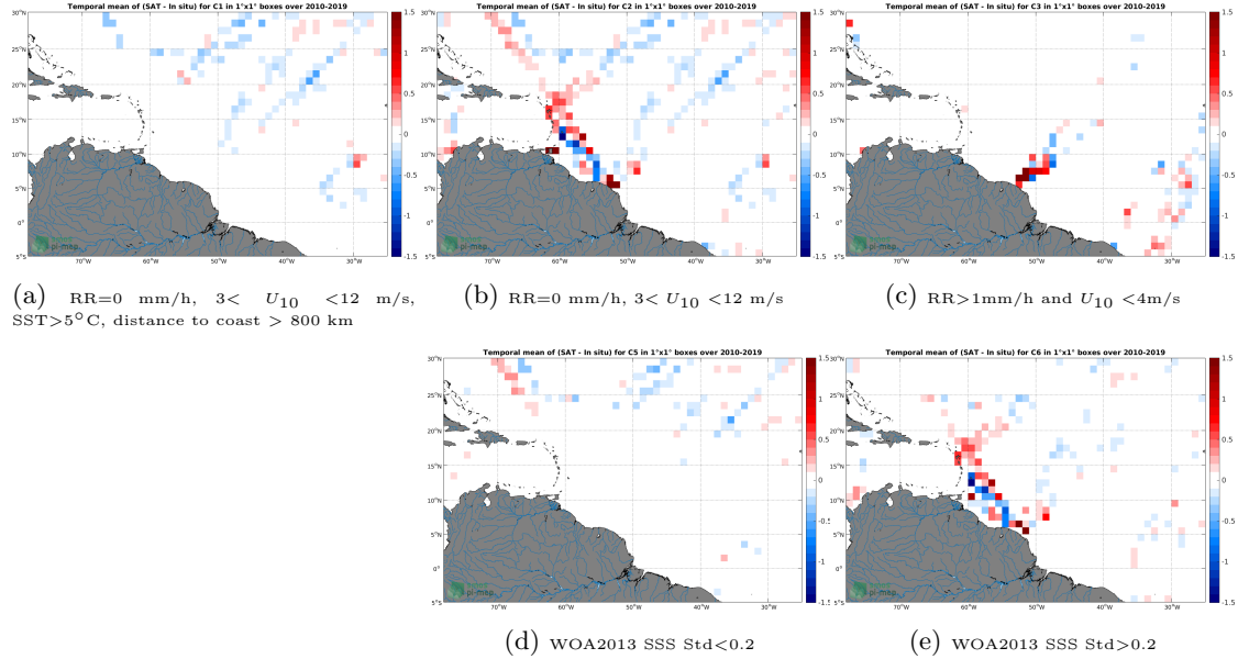
Figure 12: Temporal mean gridded over spatial boxes of size 1^{\circ}\times 1^{\circ} of \Delta\text{SSS} (SMOS SSS L3 v4 - 18 Days (CATDS-CECOS-LOCEAN) - TSG (LEGOS-DM)) for 5 different subdatasets corresponding to:RR=0 mm/h, 3 < U_{10} < 12 m/s, SST >5^{\circ}\text{C} , distance to coast > 800 km (a), RR=0 mm/h, 3 < U_{10} < 12 m/s (b), RR >1 mm/h and U_{10} < 4 m/s (c), WOA2013 SSS Std <0.2 (d), WOA2013 SSS Std >0.2 (e).
