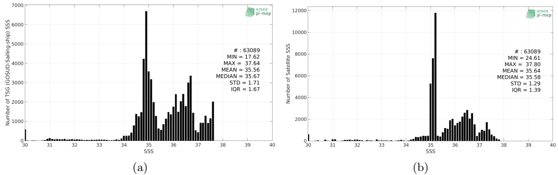
Figure 2: Histograms of SSS from TSG (GOSUD-Sailing-ship) (a) and SMOS SSS L3 v4 - 18 Days (CATDS-CECOS-LOCEAN) (b) considering all match-up pairs per bins of 0.1 over the Amazon and Orinoco river plumes Pi-MEP region and for the full satellite product period.
