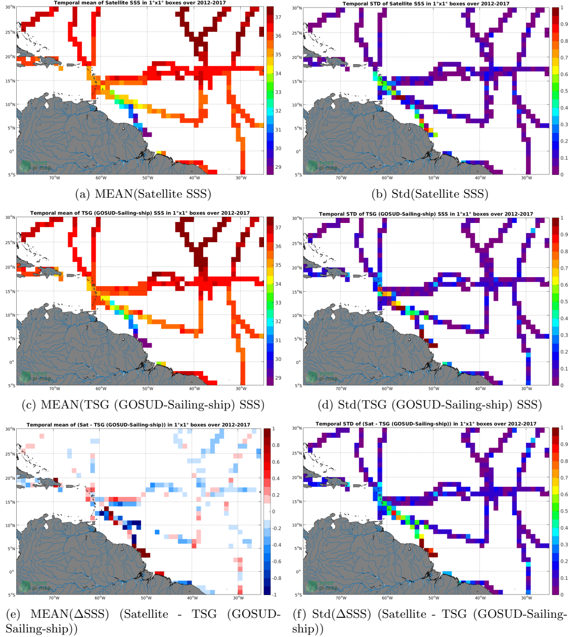
Figure 6: Temporal mean (left) and Std (right) of SSS from SMOS SSS L3 v4 - 18 Days (CATDS-CECOS-LOCEAN) (top), TSG (GOSUD-Sailing-ship) (middle), and of \Delta SSS (Satellite - TSG (GOSUD-Sailing-ship)). Only match-up pairs are used to generate these maps.
