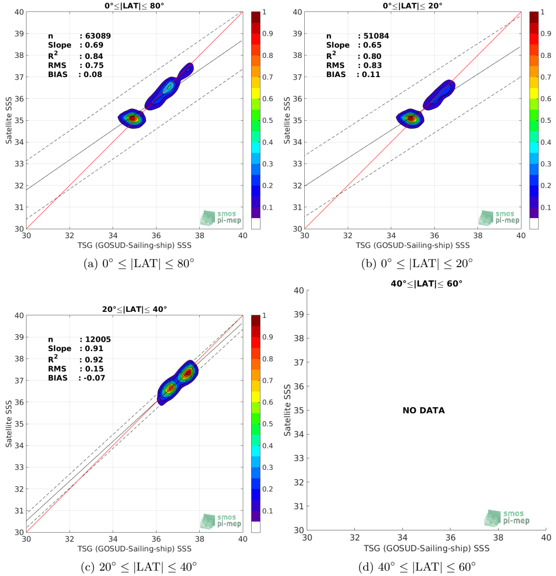
Figure 9: Contour maps of the concentration of SMOS SSS L3 v4 - 18 Days (CATDS-CECOS-LOCEAN) SSS (y-axis) versus TSG (GOSUD-Sailing-ship) SSS (x-axis) at match-up pairs for different latitude bands. For each plot, the red line shows x=y . The black thin and dashed lines indicate a linear fit through the data cloud and the \pm 95\% confidence levels, respectively. The number match-up pairs n , the slope and R^2 coefficient of the linear fit, the root mean square (RMS) and the mean bias between satellite and in situ data are indicated for each latitude band in each plots.
