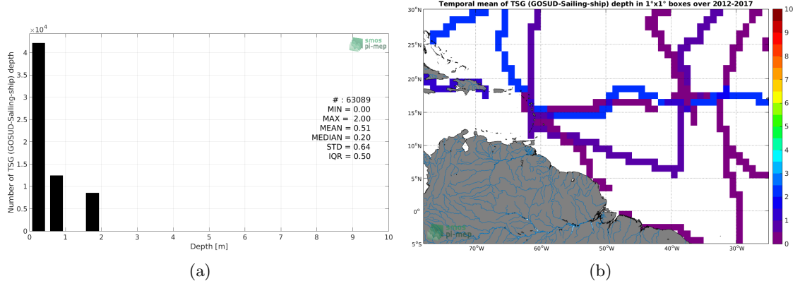
Figure 3: Histograms of the depth of the upper level SSS measurements from TSG (GOSUD-Sailing-ship) in the Match-up DataBase for the Amazon and Orinoco river plumes Pi-MEP region (a) and temporal mean spatial distribution of pressure of the in situ SSS data over 1^\circ \times 1^\circ boxes and for the full satellite product period (b).
