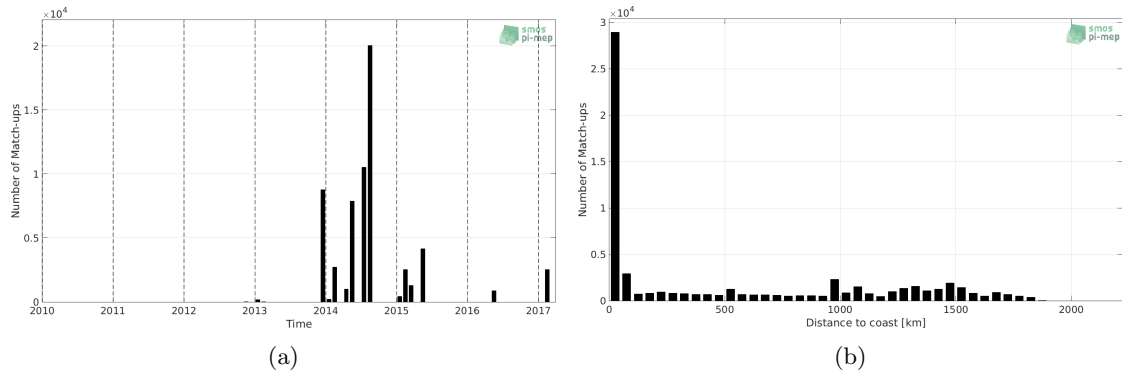
Figure 1: Number of match-ups between TSG (GOSUD-Sailing-ship) and SMOS SSS L3 v4 - 18 Days (CATDS-CECOS-LOCEAN) SSS as a function of time (a) and as function of the distance to coast (b) over the Amazon and Orinoco river plumes Pi-MEP region and for the full satellite product period.
