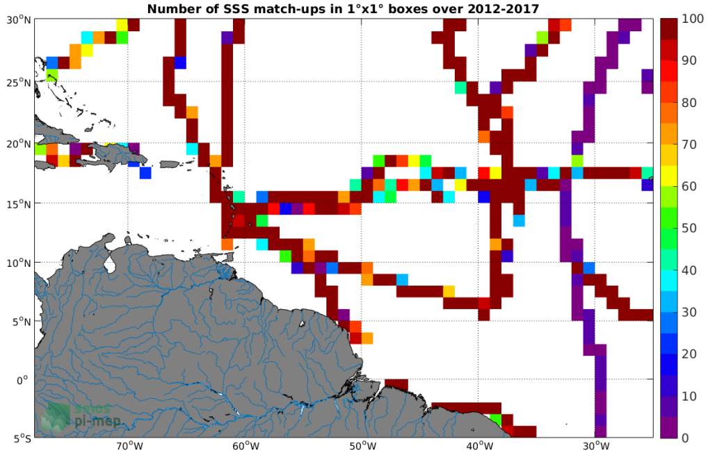
Figure 4: Number of SSS match-ups between TSG (GOSUD-Sailing-ship) SSS and the SMOS SSS L3 v4 - 18 Days (CATDS-CECOS-LOCEAN) SSS product for the Amazon and Orinoco river plumes Pi-MEP region over 1^\circ \times 1^\circ boxes and for the full satellite product period.
