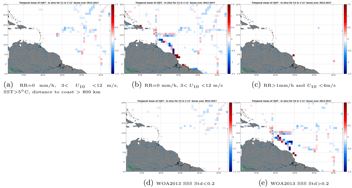
Figure 12: Temporal mean gridded over spatial boxes of size 1^\circ \times 1^\circ of \Delta SSS (SMOS SSS L3 v4 - 18 Days (CATDS-CECOS-LOCEAN) - TSG (GOSUD-Sailing-ship)) for 5 different subdatasets corresponding to: RR=0 mm/h, 3 < U_{10} < 12 m/s, SST > 5^\circ\text{C} , distance to coast > 800 km (a), RR=0 mm/h, 3 < U_{10} < 12 m/s (b), RR > 1 mm/h and U_{10} < 4 m/s (c), WOA2013 SSS Std < 0.2 (d), WOA2013 SSS Std > 0.2 (e).
