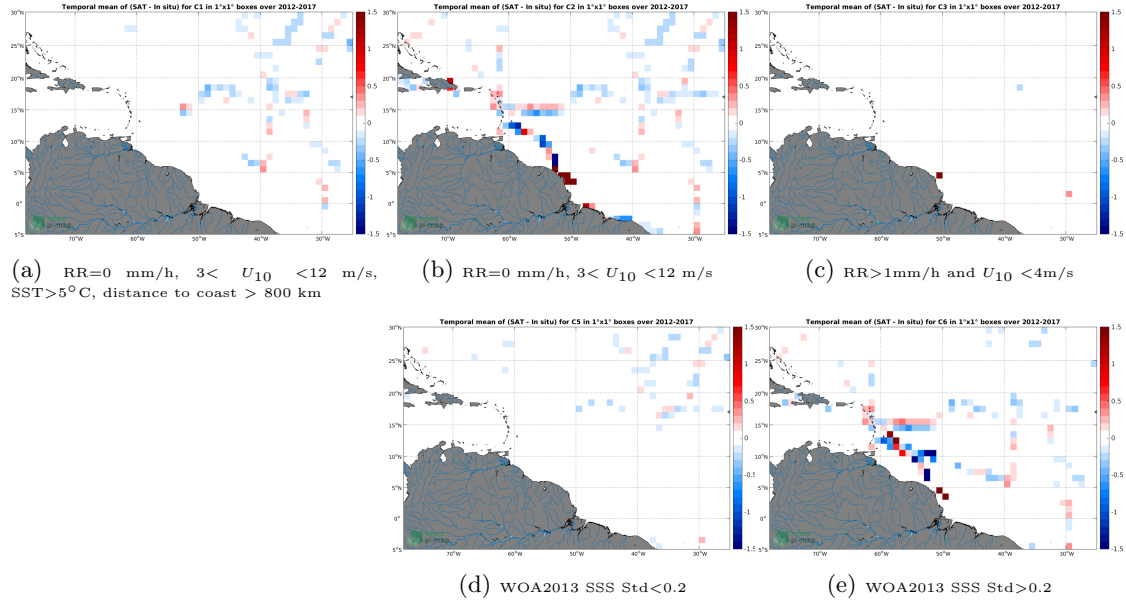
Figure 12: Temporal mean gridded over spatial boxes of size 1^{\circ}\times 1^{\circ} of \Delta SSS (SMOS-L3-CATDS-CECOS-LOCEAN-V4-18DAYS-25KM - TSG-GOSUD-Sailing-ship) for 5 different subdatasets corresponding to:RR=0 mm/h, 3 < U_{10} < 12 m/s, SST >5^{\circ}\text{C} , distance to coast > 800 km (a), RR=0 mm/h, 3 < U_{10} < 12 m/s (b), RR >1 mm/h and U_{10} < 4 m/s (c), WOA2013 SSS Std <0.2 (d), WOA2013 SSS Std >0.2 (e).
