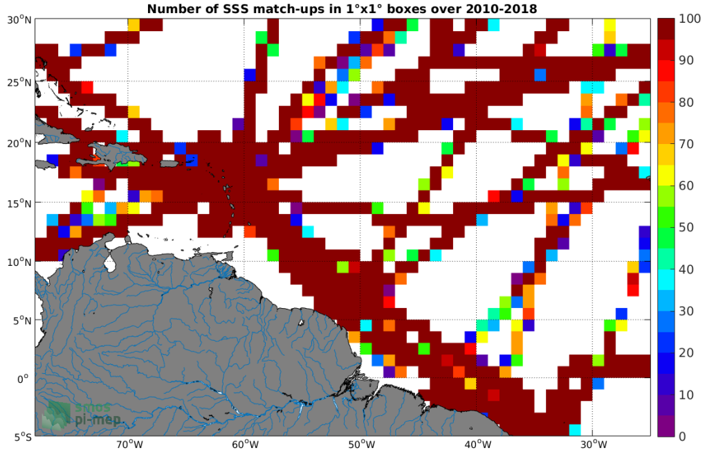
Figure 4: Number of SSS match-ups between TSG (GOSUD-Research-vessel) SSS and the SMOS SSS L3 v4 - 18 Days (CATDS-CECOS-LOCEAN) SSS product for the Amazon and Orinoco river plumes Pi-MEP region over 1^\circ \times 1^\circ boxes and for the full satellite product period.
