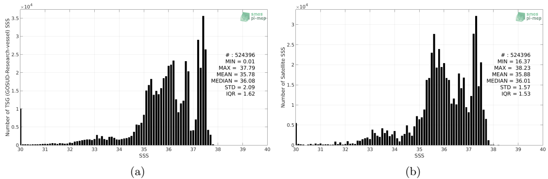
Figure 2: Histograms of SSS from TSG (GOSUD-Research-vessel) (a) and SMOS SSS L3 v4 - 18 Days (CATDS-CECOS-LOCEAN) (b) considering all match-up pairs per bins of 0.1 over the Amazon and Orinoco river plumes Pi-MEP region and for the full satellite product period.
