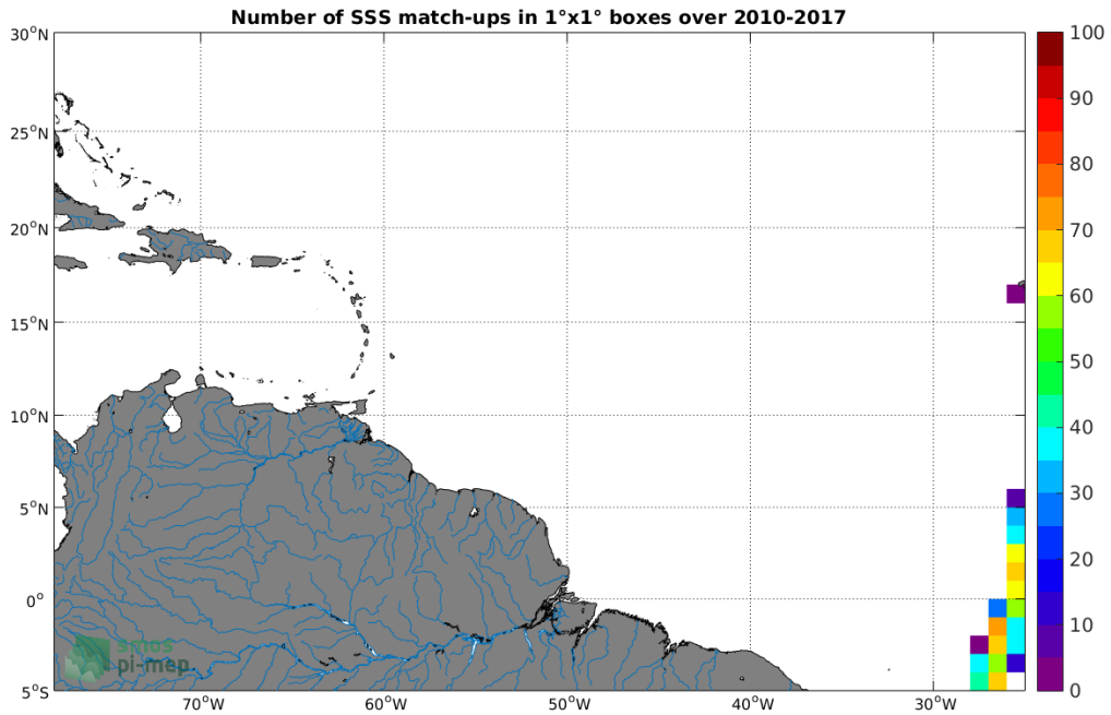
Figure 4: Number of SSS match-ups between TSG-POLARSTERN SSS and the SMOS-L3-CATDS-CECOS-LOCEAN-V3-9DAYS-25KM SSS product for the Amazon and Orinoco river plumes Pi-MEP region over 1°x1° boxes and for the full satellite product period.
