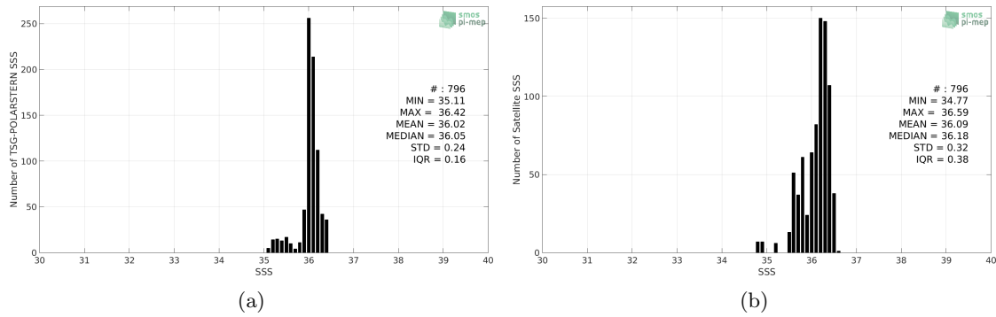
Figure 2: Histograms of SSS from TSG-POLARSTERN (a) and SMOS-L3-CATDS-CECOS-LOCEAN-V3-9DAYS-25KM (b) considering all match-up pairs per bins of 0.1 over the Amazon and Orinoco river plumes Pi-MEP region and for the full satellite product period.
