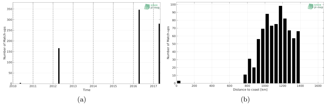
Figure 1: Number of match-ups between TSG-POLARSTERN and SMOS-L3-CATDS-CECOS-LOCEAN-V3-9DAYS-25KM SSS as a function of time (a) and as function of the distance to coast (b) over the Amazon and Orinoco river plumes Pi-MEP region and for the full satellite product period.
