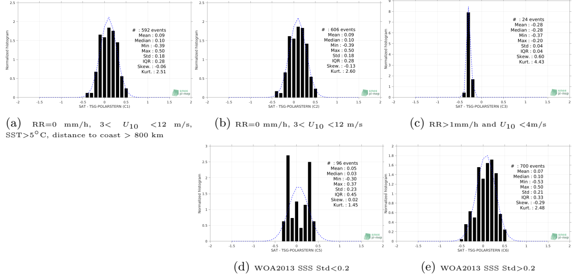
Figure 13: Normalized histogram of \Delta\text{SSS} (SMOS-L3-CATDS-CECOS-LOCEAN-V3-9DAYS-25KM - TSG-POLARSTERN) for 5 different subdatasets corresponding to: RR=0 mm/h, 3 < U_{10} < 12 m/s, SST > 5^{\circ}\text{C} , distance to coast > 800 km (a), RR=0 mm/h, 3 < U_{10} < 12 m/s (b), RR > 1\text{mm/h} and U_{10} < 4\text{m/s} (c), WOA2013 SSS Std<0.2 (d), WOA2013 SSS Std>0.2 (e).
