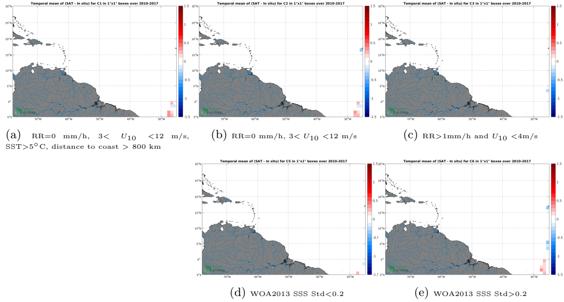
Figure 12: Temporal mean gridded over spatial boxes of size 1^\circ \times 1^\circ of \Delta SSS (SMOS-L3-CATDS-CECOS-LOCEAN-V3-9DAYS-25KM - TSG-POLARSTERN) for 5 different subdatasets corresponding to: RR=0 mm/h, 3 < U_{10} < 12 m/s, SST > 5^\circ C , distance to coast > 800 km (a), RR=0 mm/h, 3 < U_{10} < 12 m/s (b), RR > 1 mm/h and U_{10} < 4 m/s (c), WOA2013 SSS Std < 0.2 (d), WOA2013 SSS Std > 0.2 (e).
