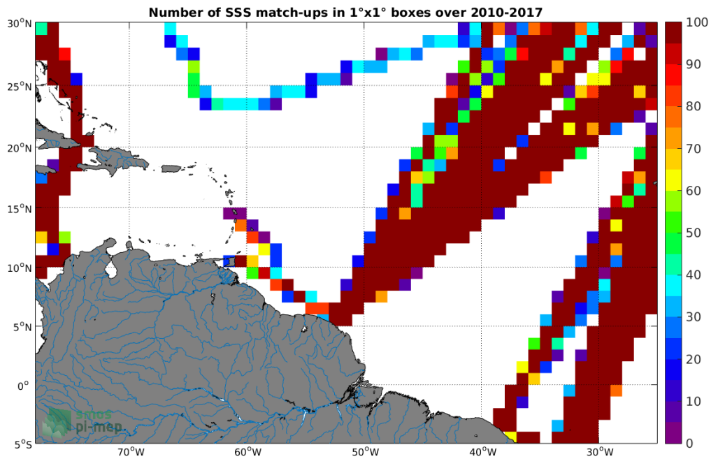
Figure 4: Number of SSS match-ups between TSG-LEGOS-DM SSS and the SMOS-L3-CATDS-CECOS-LOCEAN-V3-9DAYS-25KM SSS product for the Amazon and Orinoco river plumes Pi-MEP region over 1^\circ \times 1^\circ boxes and for the full satellite product period.
