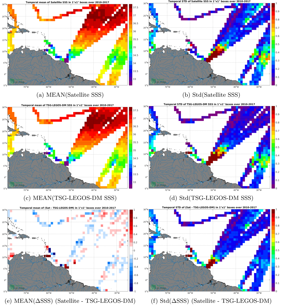
Figure 6: Temporal mean (left) and Std (right) of SSS from SMOS-L3-CATDS-CECOS-LOCEAN-V3-9DAYS-25KM (top), TSG-LEGOS-DM (middle), and of \Delta SSS (Satellite - TSG-LEGOS-DM). Only match-up pairs are used to generate these maps.
