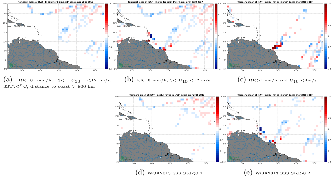
Figure 12: Temporal mean gridded over spatial boxes of size 1^\circ \times 1^\circ of \Delta SSS (SMOS-L3-CATDS-CECOS-LOCEAN-V3-9DAYS-25KM - TSG-LEGOS-DM) for 5 different subdatasets corresponding to: RR=0 mm/h, 3 < U_{10} < 12 m/s, SST > 5^\circ C , distance to coast > 800 km (a), RR=0 mm/h, 3 < U_{10} < 12 m/s (b), RR > 1 mm/h and U_{10} < 4 m/s (c), WOA2013 SSS Std < 0.2 (d), WOA2013 SSS Std > 0.2 (e).
