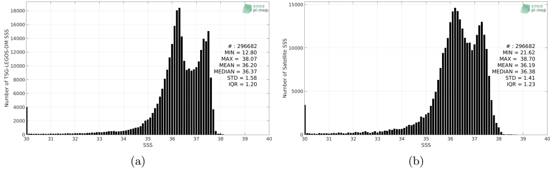
Figure 2: Histograms of SSS from TSG-LEGOS-DM (a) and SMOS-L3-CATDS-CECOS-LOCEAN-V3-9DAYS-25KM (b) considering all match-up pairs per bins of 0.1 over the Amazon and Orinoco river plumes Pi-MEP region and for the full satellite product period.
