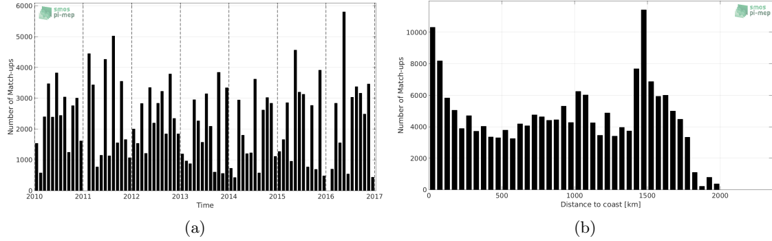
Figure 1: Number of match-ups between TSG-LEGOS-DM and SMOS-L3-CATDS-CECOS-LOCEAN-V3-9DAYS-25KM SSS as a function of time (a) and as function of the distance to coast (b) over the Amazon and Orinoco river plumes Pi-MEP region and for the full satellite product period.
