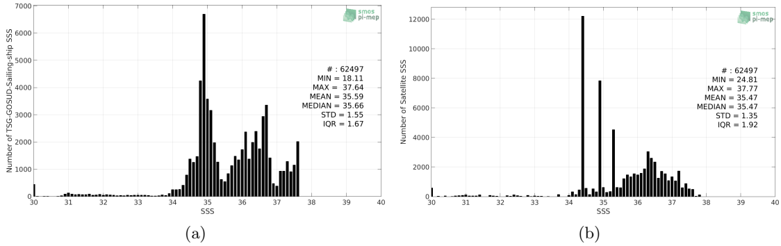
Figure 2: Histograms of SSS from TSG-GOSUD-Sailing-ship (a) and SMOS-L3-CATDS-CECOS-LOCEAN-V3-9DAYS-25KM (b) considering all match-up pairs per bins of 0.1 over the Amazon and Orinoco river plumes Pi-MEP region and for the full satellite product period.
