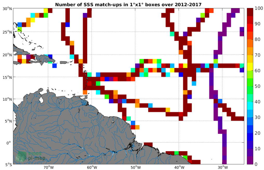
Figure 4: Number of SSS match-ups between TSG-GOSUD-Sailing-ship SSS and the SMOS-L3-CATDS-CECOS-LOCEAN-V3-9DAYS-25KM SSS product for the Amazon and Orinoco river plumes Pi-MEP region over 1^\circ \times 1^\circ boxes and for the full satellite product period.
