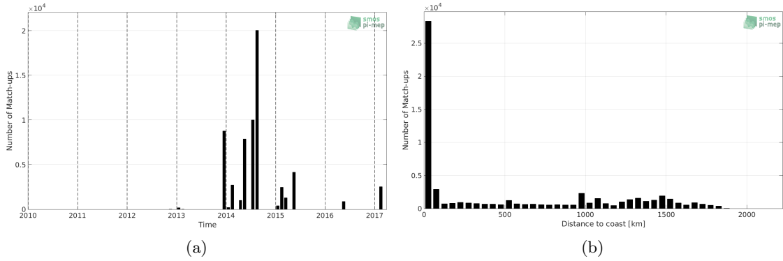
Figure 1: Number of match-ups between TSG-GOSUD-Sailing-ship and SMOS-L3-CATDS-CECOS-LOCEAN-V3-9DAYS-25KM SSS as a function of time (a) and as function of the distance to coast (b) over the Amazon and Orinoco river plumes Pi-MEP region and for the full satellite product period.
