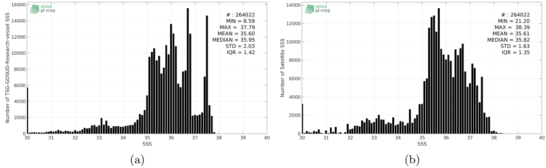
Figure 2: Histograms of SSS from TSG-GOSUD-Research-vessel (a) and SMOS-L3-CATDS-CECOS-LOCEAN-V3-9DAYS-25KM (b) considering all match-up pairs per bins of 0.1 over the Amazon and Orinoco river plumes Pi-MEP region and for the full satellite product period.
