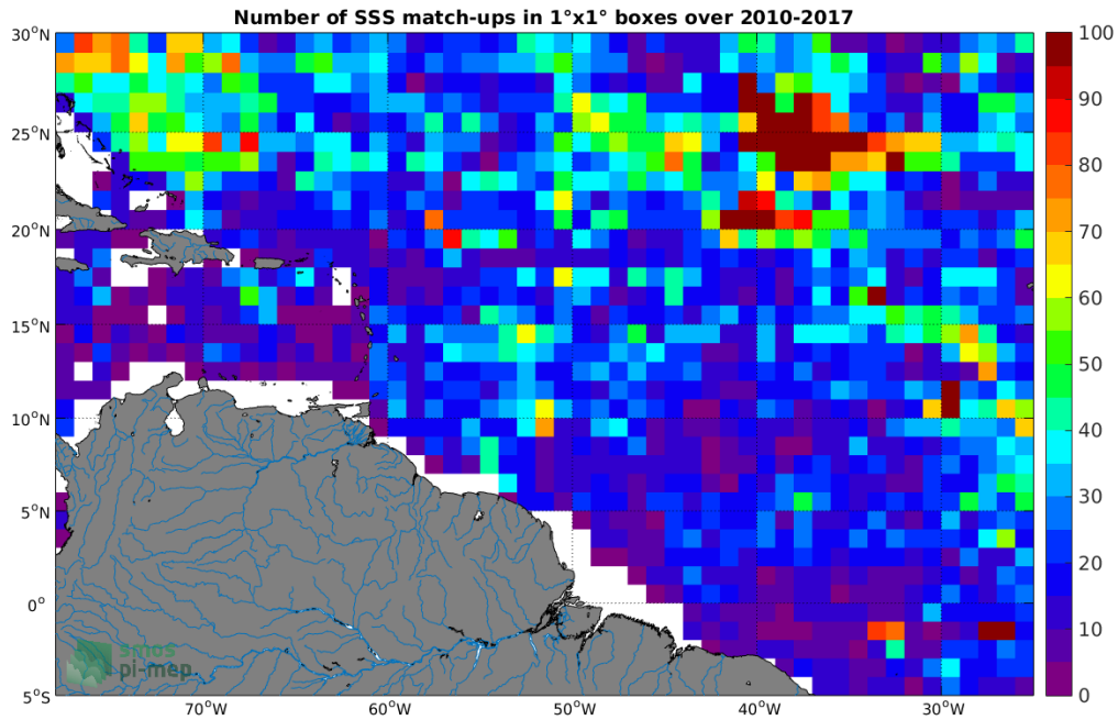
Figure 4: Number of SSS match-ups between Argo SSS and the SMOS-L3-CATDS-CECOS-LOCEAN-V3-9DAYS-25KM SSS product for the Amazon and Orinoco river plumes Pi-MEP region over 1^\circ \times 1^\circ boxes and for the full satellite product period.
