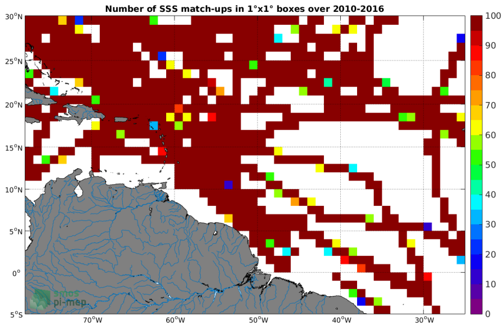
Figure 4: Number of SSS match-ups between TSG-SAMOS SSS and the SMOS-L3-CATDS-CECOS-LOCEAN-V3-18DAYS-25KM SSS product for the Amazon and Orinoco river plumes Pi-MEP region over 1^\circ \times 1^\circ boxes and for the full satellite product period.
