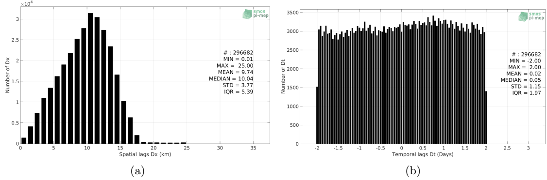
Figure 5: Histograms of the spatial (a) and temporal (b) lags between the time of the TSG-LEGOS-DM measurements and the date of the corresponding SMOS-L3-CATDS-CECOS-LOCEAN-V3-18DAYS-25KM SSS product.
