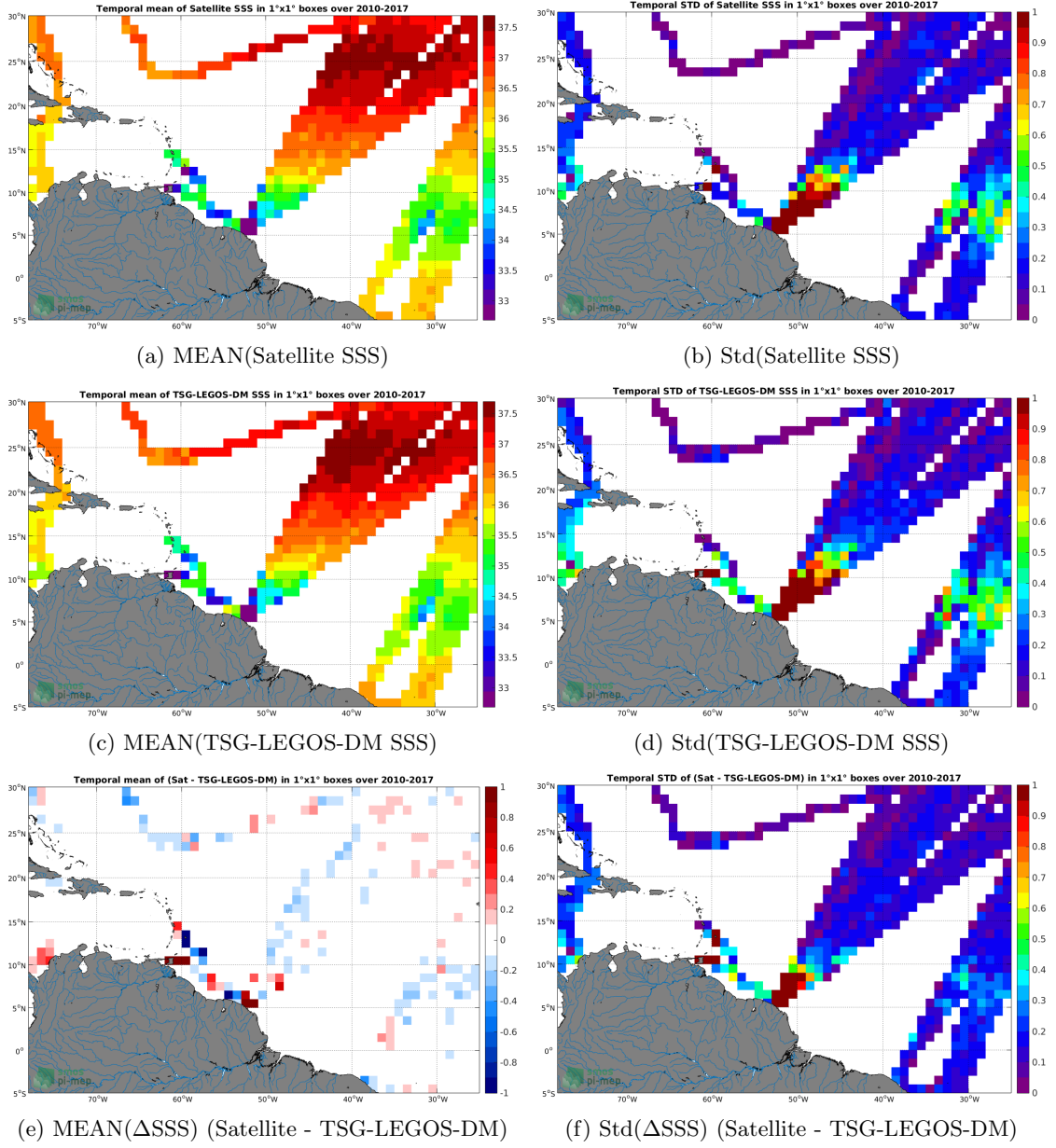
Figure 6: Temporal mean (left) and Std (right) of SSS from SMOS-L3-CATDS-CECOS-LOCEAN-V3-18DAYS-25KM (top), TSG-LEGOS-DM (middle), and of \Delta SSS (Satellite - TSG-LEGOS-DM). Only match-up pairs are used to generate these maps.
