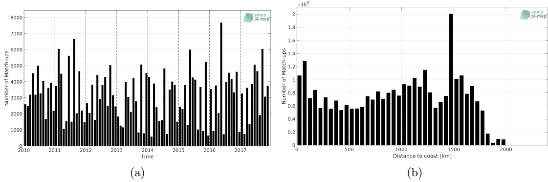
Figure 1: Number of match-ups between TSG-LEGOS-DM and SMOS-L3-CATDS-CECOS-LOCEAN-V3-18DAYS-25KM SSS as a function of time (a) and as function of the distance to coast (b) over the Amazon and Orinoco river plumes Pi-MEP region and for the full satellite product period.
