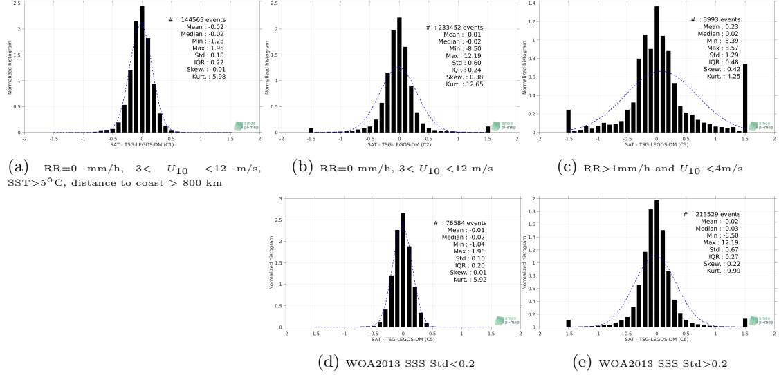
Figure 13: Normalized histogram of \Delta SSS (SMOS-L3-CATDS-CECOS-LOCEAN-V3-18DAYS-25KM - TSG-LEGOS-DM) for 5 different subdatasets corresponding to: RR=0 mm/h, 3 < U_{10} < 12 m/s, SST>5°C, distance to coast > 800 km (a), RR=0 mm/h, 3 < U_{10} < 12 m/s (b), RR>1mm/h and U_{10} < 4 m/s (c), WOA2013 SSS Std<0.2 (d), WOA2013 SSS Std>0.2 (e).
