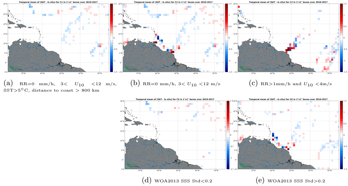
Figure 12: Temporal mean gridded over spatial boxes of size 1^\circ \times 1^\circ of \Delta SSS (SMOS-L3-CATDS-CECOS-LOCEAN-V3-18DAYS-25KM - TSG-LEGOS-DM) for 5 different subdatasets corresponding to: RR=0 mm/h, 3 < U_{10} < 12 m/s, SST > 5^\circ C , distance to coast > 800 km (a), RR=0 mm/h, 3 < U_{10} < 12 m/s (b), RR > 1 mm/h and U_{10} < 4 m/s (c), WOA2013 SSS Std < 0.2 (d), WOA2013 SSS Std > 0.2 (e).
