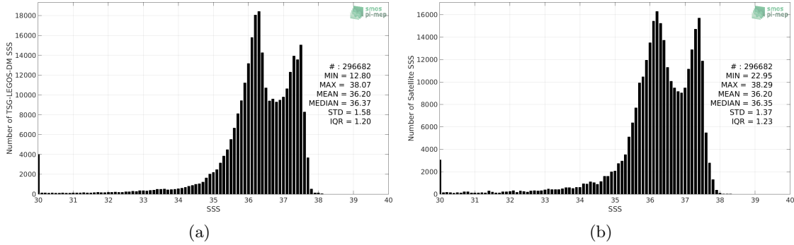
Figure 2: Histograms of SSS from TSG-LEGOS-DM (a) and SMOS-L3-CATDS-CECOS-LOCEAN-V3-18DAYS-25KM (b) considering all match-up pairs per bins of 0.1 over the Amazon and Orinoco river plumes Pi-MEP region and for the full satellite product period.
