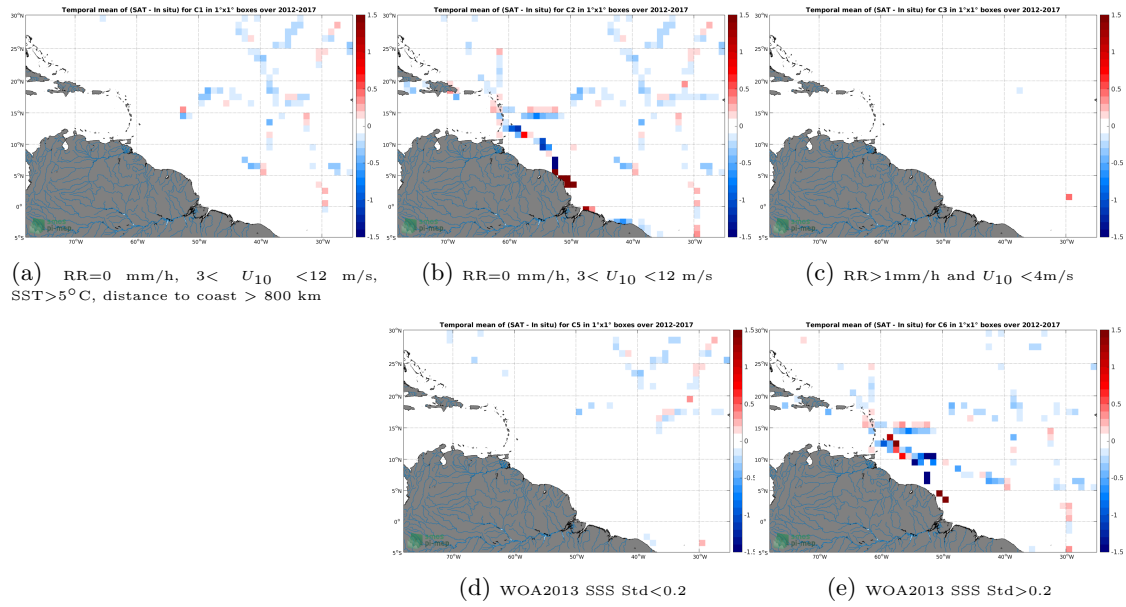
Figure 12: Temporal mean gridded over spatial boxes of size 1^\circ \times 1^\circ of \Delta SSS (SMOS-L3-CATDS-CECOS-LOCEAN-V3-18DAYS-25KM - TSG-GOSUD-Sailing-ship) for 5 different subdatasets corresponding to: RR=0 mm/h, 3 < U_{10} < 12 m/s, SST > 5^\circ C , distance to coast > 800 km (a), RR=0 mm/h, 3 < U_{10} < 12 m/s (b), RR > 1 mm/h and U_{10} < 4 m/s (c), WOA2013 SSS Std < 0.2 (d), WOA2013 SSS Std > 0.2 (e).
