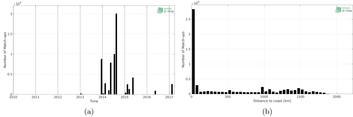
Figure 1: Number of match-ups between TSG-GOSUD-Sailing-ship and SMOS-L3-CATDS-CECOS-LOCEAN-V3-18DAYS-25KM SSS as a function of time (a) and as function of the distance to coast (b) over the Amazon and Orinoco river plumes Pi-MEP region and for the full satellite product period.
