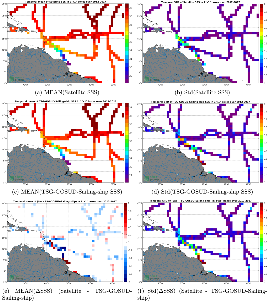
Figure 6: Temporal mean (left) and Std (right) of SSS from SMOS-L3-CATDS-CECOS-LOCEAN-V3-18DAYS-25KM (top), TSG-GOSUD-Sailing-ship (middle), and of \Delta SSS (Satellite - TSG-GOSUD-Sailing-ship). Only match-up pairs are used to generate these maps.
