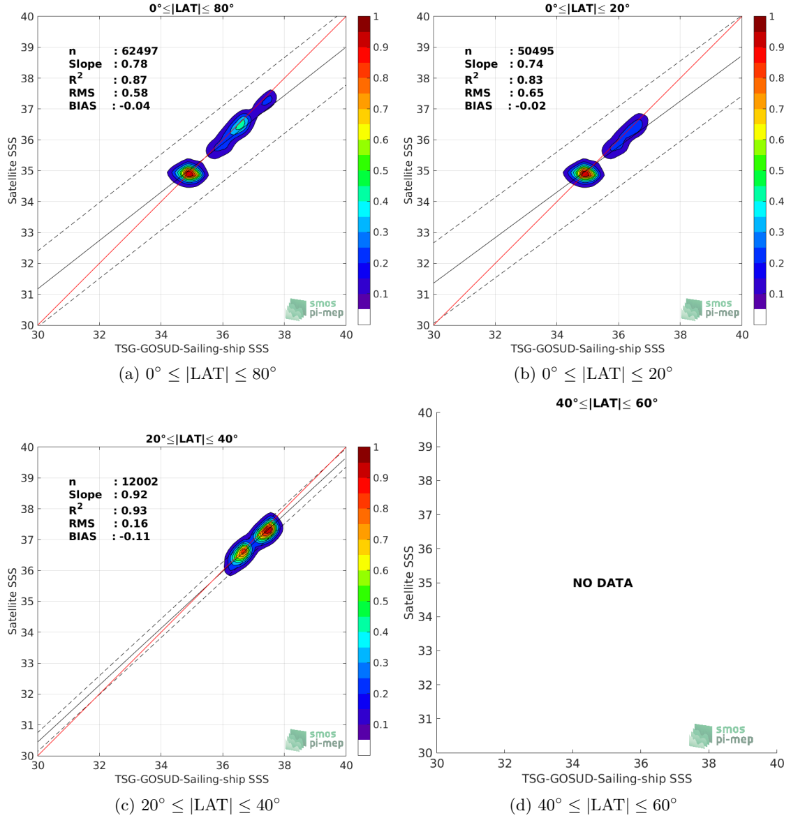
Figure 9: Contour maps of the concentration of SMOS-L3-CATDS-CECOS-LOCEAN-V3-18DAYS-25KM SSS (y-axis) versus TSG-GOSUD-Sailing-ship SSS (x-axis) at match-up pairs for different latitude bands. For each plot, the red line shows x=y . The black thin and dashed lines indicate a linear fit through the data cloud and the \pm 95\% confidence levels, respectively. The number match-up pairs n , the slope and R^2 coefficient of the linear fit, the root mean square (RMS) and the mean bias between satellite and in situ data are indicated for each latitude band in each plots.
