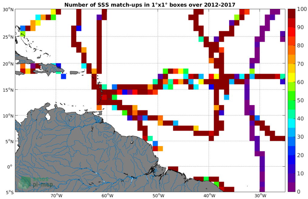
Figure 4: Number of SSS match-ups between TSG-GOSUD-Sailing-ship SSS and the SMOS-L3-CATDS-CECOS-LOCEAN-V3-18DAYS-25KM SSS product for the Amazon and Orinoco river plumes Pi-MEP region over 1^\circ \times 1^\circ boxes and for the full satellite product period.
