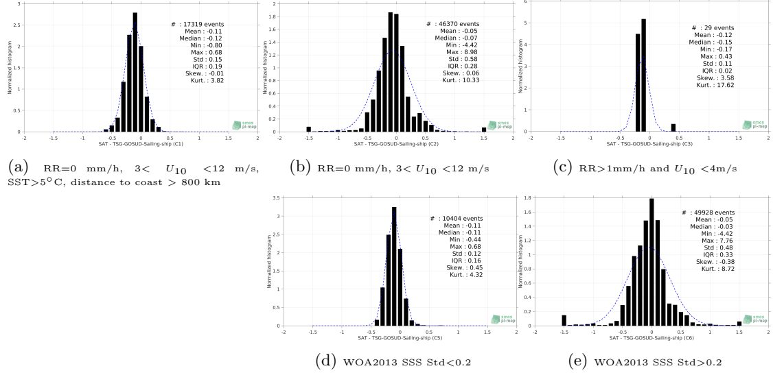
Figure 13: Normalized histogram of \Delta\text{SSS} (SMOS-L3-CATDS-CECOS-LOCEAN-V3-18DAYS-25KM - TSG-GOSUD-Sailing-ship) for 5 different subdatasets corresponding to: RR=0 mm/h, 3 < U_{10} < 12 m/s, SST > 5^\circ\text{C} , distance to coast > 800 km (a), RR=0 mm/h, 3 < U_{10} < 12 m/s (b), RR > 1\text{mm/h} and U_{10} < 4\text{m/s} (c), WOA2013 SSS Std < 0.2 (d), WOA2013 SSS Std > 0.2 (e).
