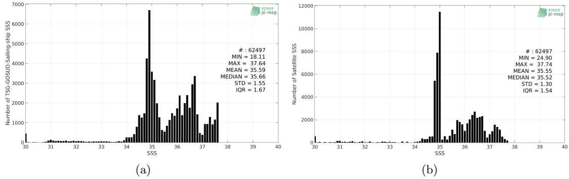
Figure 2: Histograms of SSS from TSG-GOSUD-Sailing-ship (a) and SMOS-L3-CATDS-CECOS-LOCEAN-V3-18DAYS-25KM (b) considering all match-up pairs per bins of 0.1 over the Amazon and Orinoco river plumes Pi-MEP region and for the full satellite product period.
