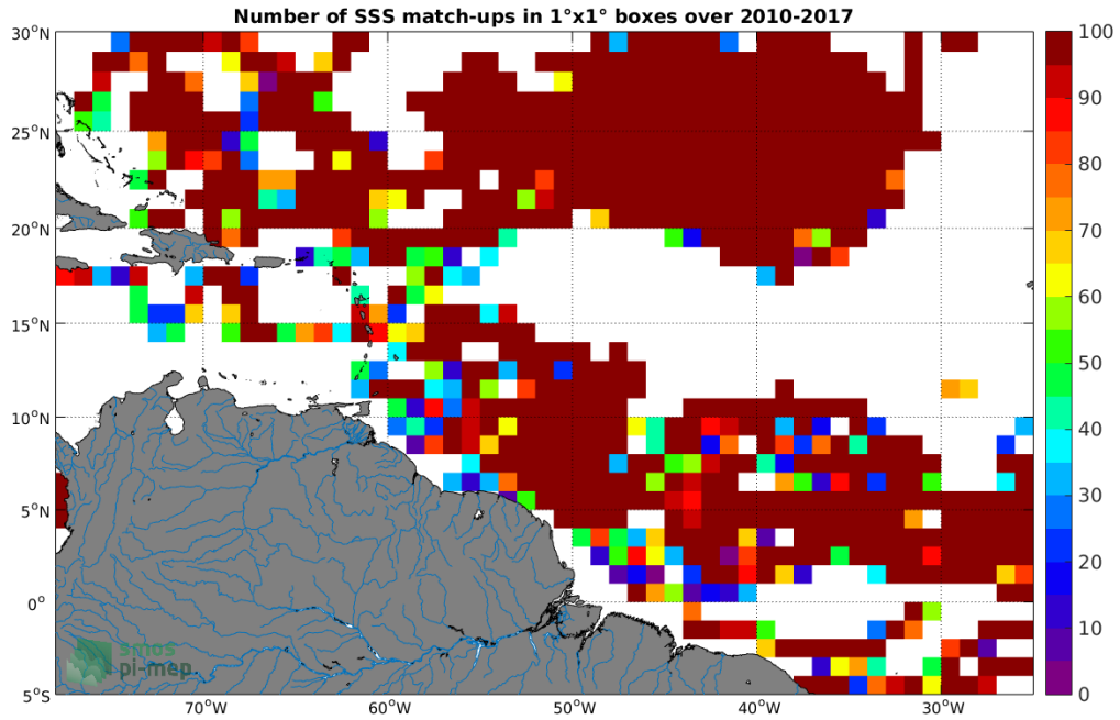
Figure 3: Number of SSS match-ups between Surface drifters SSS and the SMOS-L3-CATDS-CECOS-LOCEAN-V3-18DAYS-25KM SSS product for the Amazon and Orinoco river plumes Pi-MEP region over 1°x1° boxes and for the full satellite product period.
