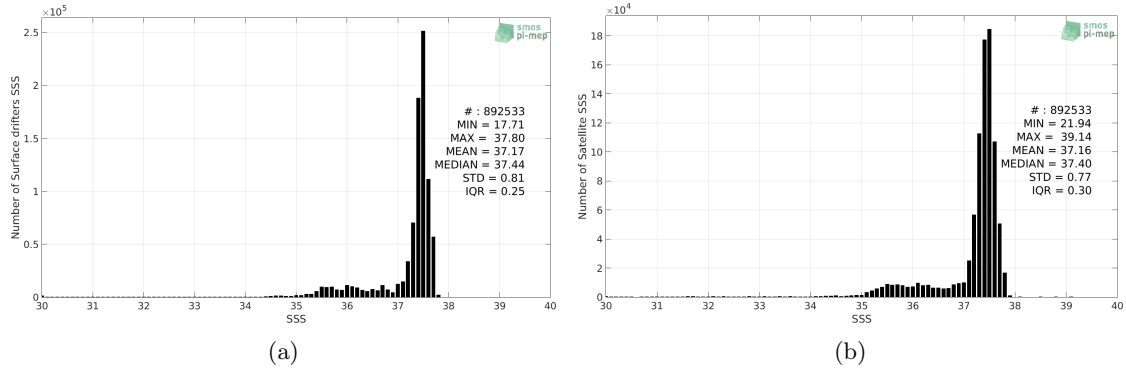
Figure 2: Histograms of SSS from Surface drifters (a) and SMOS-L3-CATDS-CECOS-LOCEAN-V3-18DAYS-25KM (b) considering all match-up pairs per bins of 0.1 over the Amazon and Orinoco river plumes Pi-MEP region and for the full satellite product period.
