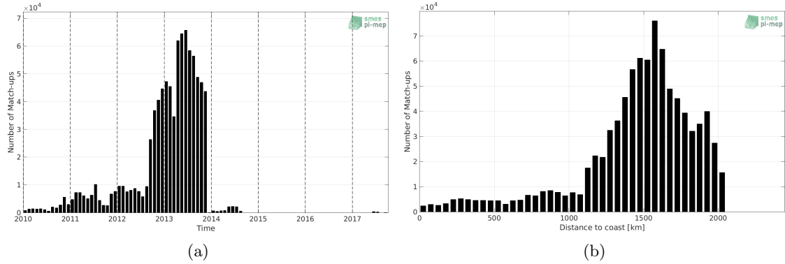
Figure 1: Number of match-ups between Surface drifters and SMOS-L3-CATDS-CECOS-LOCEAN-V3-18DAYS-25KM SSS as a function of time (a) and as function of the distance to coast (b) over the Amazon and Orinoco river plumes Pi-MEP region and for the full satellite product period.
