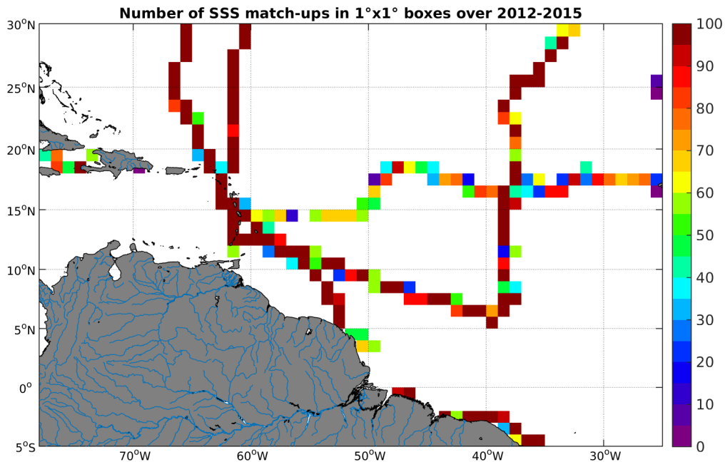
Figure 4: Number of SSS match-ups between TSG-GOSUD-Sailing-ship SSS and the SMOS-L3-CATDS-CECOS-LOCEAN-V2.1-9DAYS-25KM SSS product for the Amazon and Orinoco river plumes Pi-MEP region over 1°x1° boxes and for the full satellite product period.
