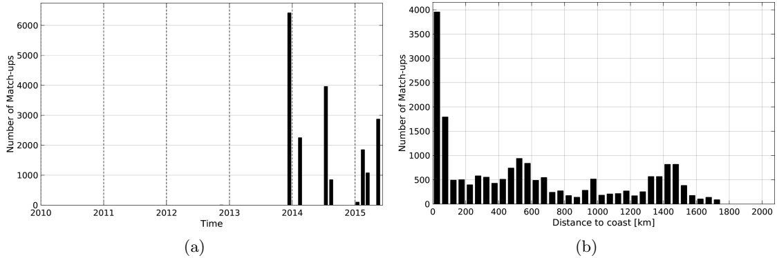
Figure 1: Number of match-ups between TSG-GOSUD-Sailing-ship and SMOS-L3-CATDS-CECOS-LOCEAN-V2.1-9DAYS-25KM SSS as a function of time (a) and as function of the distance to coast (b) over the Amazon and Orinoco river plumes Pi-MEP region and for the full satellite product period.
