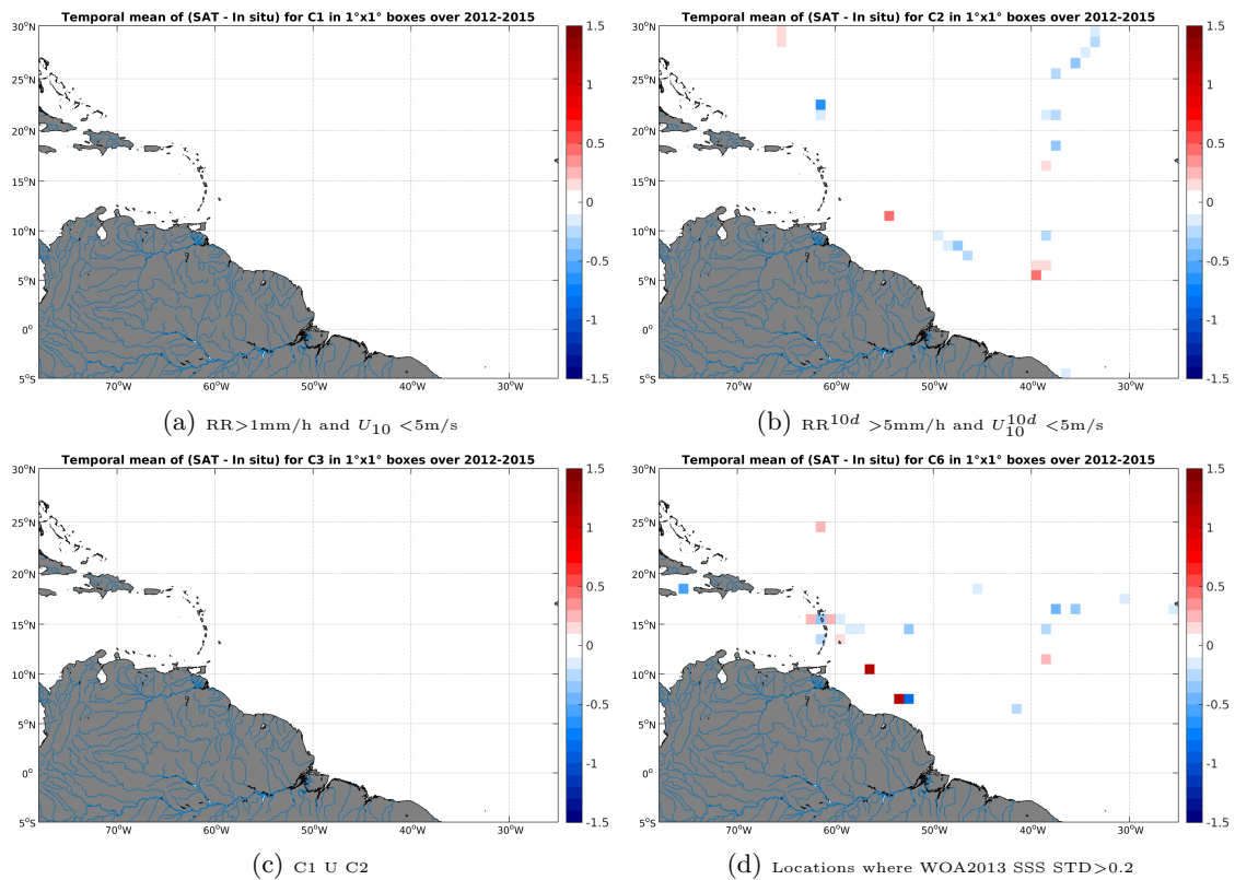
Figure 12: Temporal mean gridded over spatial boxes of size 1^\circ \times 1^\circ of \Delta SSS (SMOS-L3-CATDS-CECOS-LOCEAN-V2.1-9DAYS-25KM - TSG-GOSUD-Sailing-ship) for 4 different subdatasets corresponding to:RR >1 mm/h and U_{10} < 5 m/s (a), RR^{10d} > 5 mm/h and U_{10}^{10d} < 5 m/s (b), C1 U C2 (c),Locations where WOA2013 SSS STD >0.2 (d).
