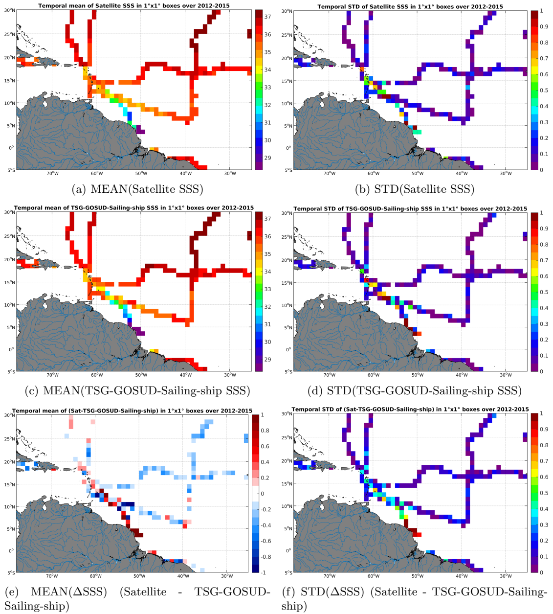
Figure 6: Temporal mean (left) and STD (right) of SSS from SMOS-L3-CATDS-CECOS-LOCEAN-V2.1-9DAYS-25KM (top), TSG-GOSUD-Sailing-ship (middle), and of \Delta SSS (Satellite - TSG-GOSUD-Sailing-ship). Only match-up pairs are used to generate these maps.
