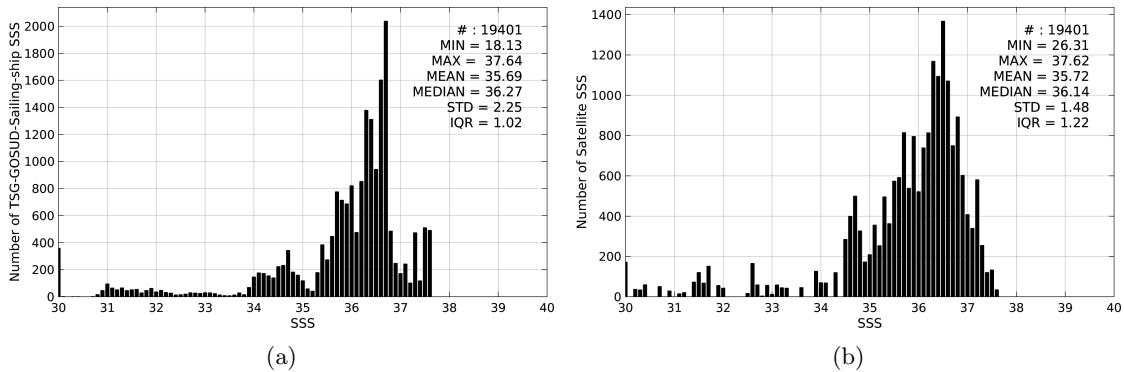
Figure 2: Histograms of SSS from TSG-GOSUD-Sailing-ship (a) and SMOS-L3-CATDS-CECOS-LOCEAN-V2.1-9DAYS-25KM (b) considering all match-up pairs per bins of 0.1 over the Amazon and Orinoco river plumes Pi-MEP region and for the full satellite product period.
