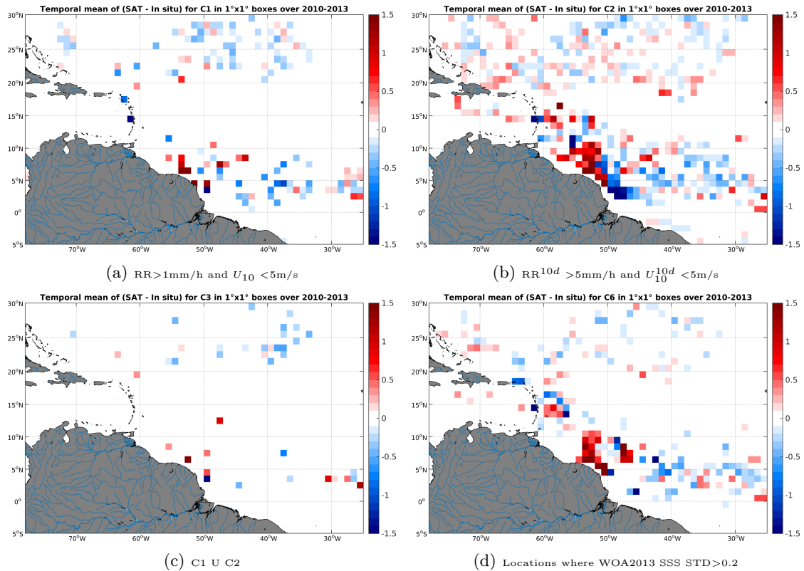
Figure 11: Temporal mean gridded over spatial boxes of size 1^\circ \times 1^\circ of \Delta SSS (SMOS-L3-CATDS-CECOS-LOCEAN-V2.1-9DAYS-25KM - Surface drifters) for 4 different subdatasets corresponding to: RR > 1\text{mm/h} and U_{10} < 5\text{m/s} (a), RR^{10d} > 5\text{mm/h} and U_{10}^{10d} < 5\text{m/s} (b), C1 U C2 (c), Locations where WOA2013 SSS STD > 0.2 (d).
