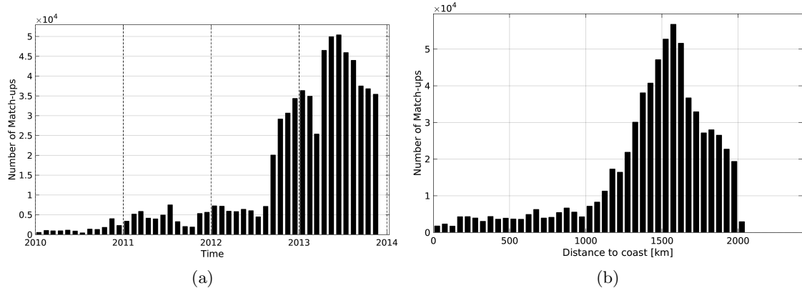
Figure 1: Number of match-ups between Surface drifters and SMOS-L3-CATDS-CECOS-LOCEAN-V2.1-9DAYS-25KM SSS as a function of time (a) and as function of the distance to coast (b) over the Amazon and Orinoco river plumes Pi-MEP region and for the full satellite product period.
