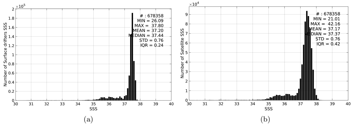
Figure 2: Histograms of SSS from Surface drifters (a) and SMOS-L3-CATDS-CECOS-LOCEAN-V2.1-9DAYS-25KM (b) considering all match-up pairs per bins of 0.1 over the Amazon and Orinoco river plumes Pi-MEP region and for the full satellite product period.
