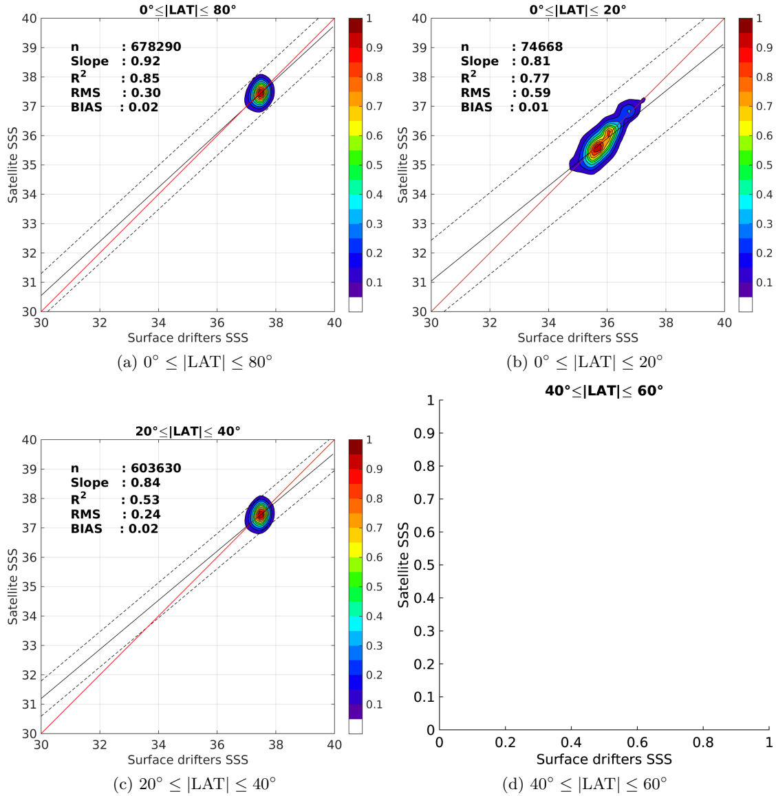
Figure 8: Contour maps of the concentration of SMOS-L3-CATDS-CECOS-LOCEAN-V2.1-9DAYS-25KM SSS (y-axis) versus Surface drifters SSS (x-axis) at match-up pairs for different latitude bands. For each plot, the red line shows x=y . The black thin and dashed lines indicate a linear fit through the data cloud and the \pm 95\% confidence levels, respectively. The number match-up pairs n , the slope and R^2 coefficient of the linear fit, the root mean square (RMS) and the mean bias between satellite and in situ data are indicated for each latitude band in each plots.
