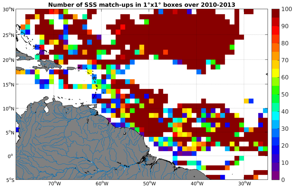
Figure 3: Number of SSS match-ups between Surface drifters SSS and the SMOS-L3-CATDS-CECOS-LOCEAN-V2.1-9DAYS-25KM SSS product for the Amazon and Orinoco river plumes Pi-MEP region over 1^{\circ} \times 1^{\circ} boxes and for the full satellite product period.
