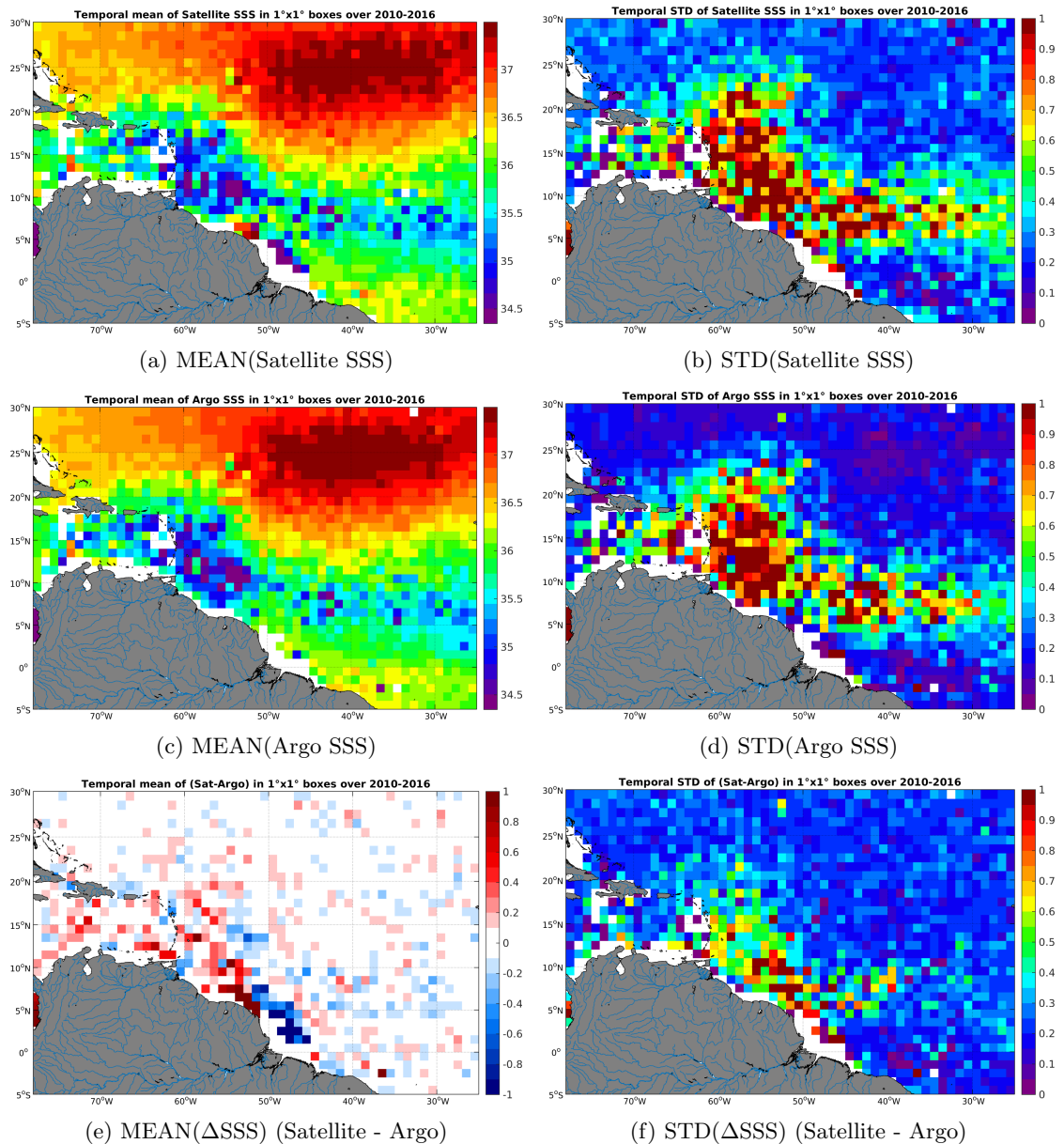
Figure 6: Temporal mean (left) and STD (right) of SSS from SMOS-L3-CATDS-CECOS-LOCEAN-V2.1-9DAYS-25KM (top), Argo (middle), and of \Delta SSS (Satellite - Argo). Only match-up pairs are used to generate these maps.
