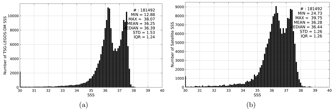
Figure 2: Histograms of SSS from TSG-LEGOS-DM (a) and SMOS-L3-CATDS-CECOS-LOCEAN-V2-9DAYS-25KM (b) considering all match-up pairs per bins of 0.1 over the Amazon and Orinoco river plumes Pi-MEP region and for the full satellite product period.
