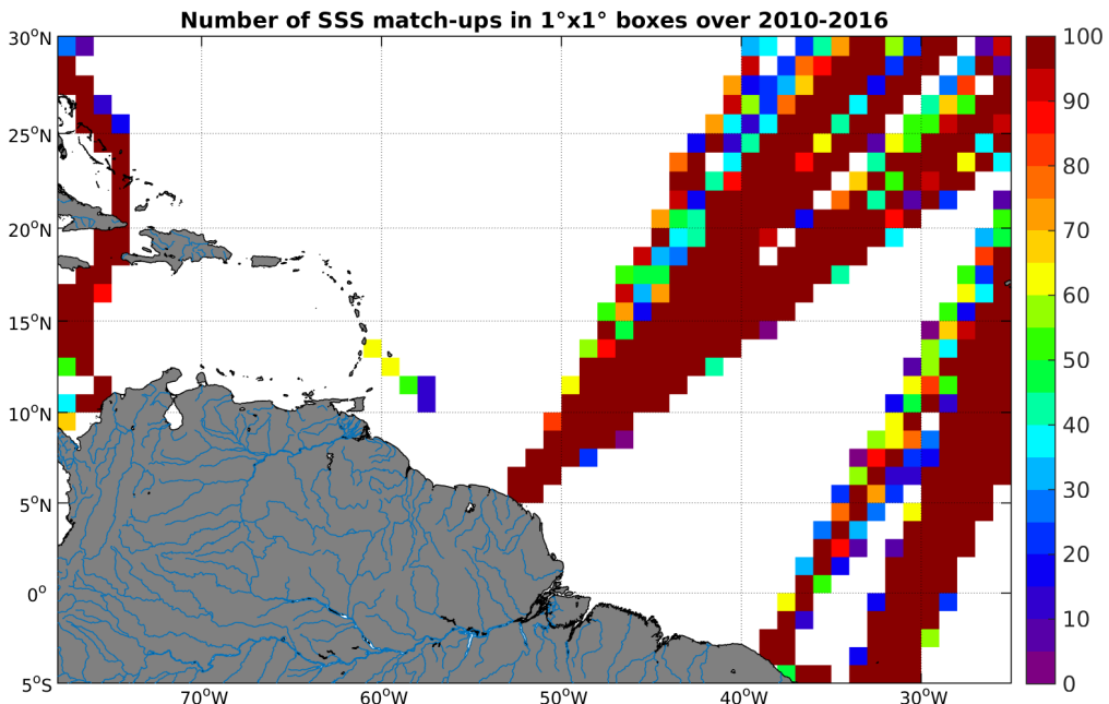
Figure 4: Number of SSS match-ups between TSG-LEGOS-DM SSS and the SMOS-L3-CATDS-CECOS-LOCEAN-V2-9DAYS-25KM SSS product for the Amazon and Orinoco river plumes Pi-MEP region over 1^\circ \times 1^\circ boxes and for the full satellite product period.
