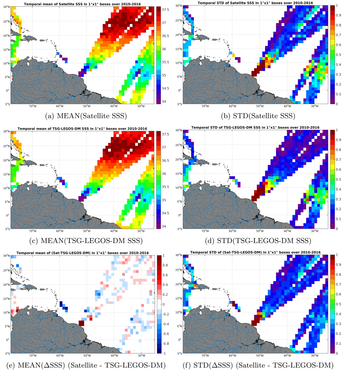
Figure 6: Temporal mean (left) and STD (right) of SSS from SMOS-L3-CATDS-CECOS-LOCEAN-V2-9DAYS-25KM (top), TSG-LEGOS-DM (middle), and of \Delta SSS (Satellite - TSG-LEGOS-DM). Only match-up pairs are used to generate these maps.
