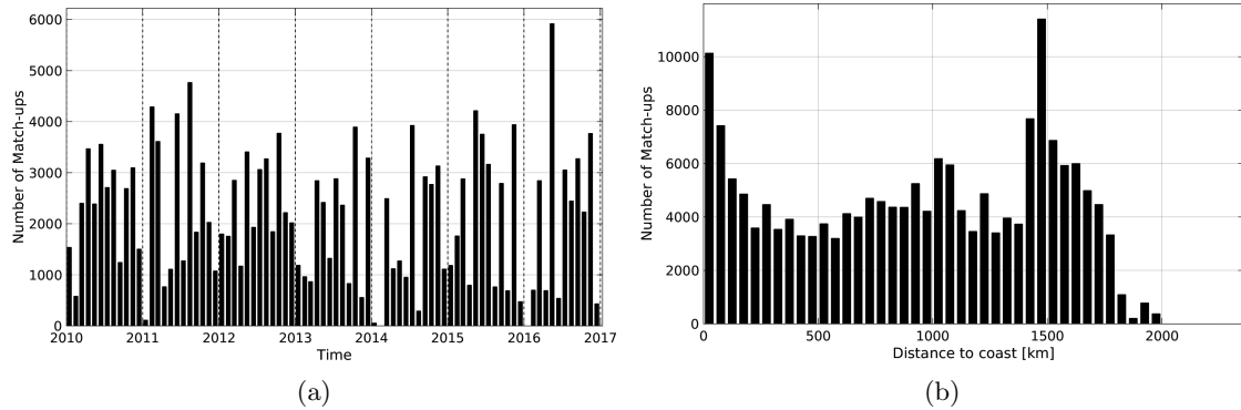
Figure 1: Number of match-ups between TSG-LEGOS-DM and SMOS-L3-CATDS-CECOS-LOCEAN-V2-9DAYS-25KM SSS as a function of time (a) and as function of the distance to coast (b) over the Amazon and Orinoco river plumes Pi-MEP region and for the full satellite product period.
