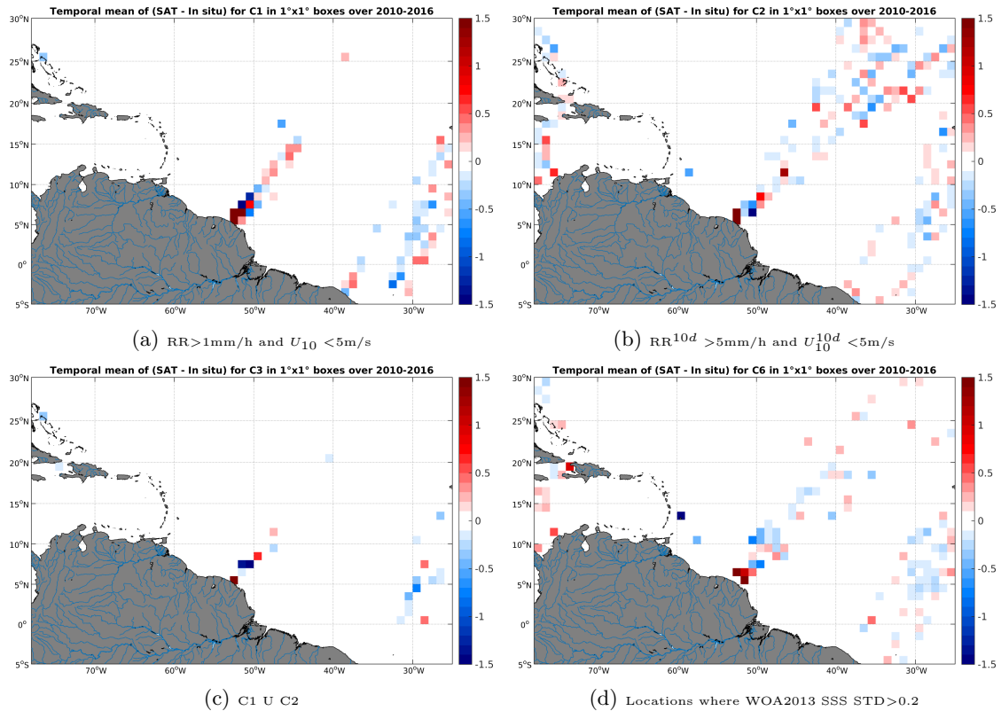
Figure 12: Temporal mean gridded over spatial boxes of size 1^\circ \times 1^\circ of \Delta SSS (SMOS-L3-CATDS-CECOS-LOCEAN-V2-9DAYS-25KM - TSG-LEGOS-DM) for 4 different subdatasets corresponding to:RR >1 mm/h and U_{10} < 5 m/s (a), RR ^{10d} > 5 mm/h and U_{10}^{10d} < 5 m/s (b), C1 U C2 (c),Locations where WOA2013 SSS STD >0.2 (d).
