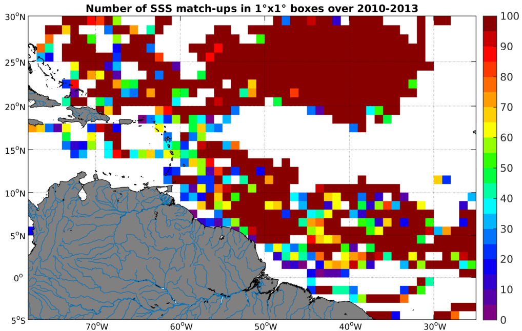
Figure 3: Number of SSS match-ups between Surface drifters SSS and the SMOS-L3-CATDS-CECOS-LOCEAN-V2-9DAYS-25KM SSS product for the Amazon and Orinoco river plumes Pi-MEP region over 1^{\circ} \times 1^{\circ} boxes and for the full satellite product period.
