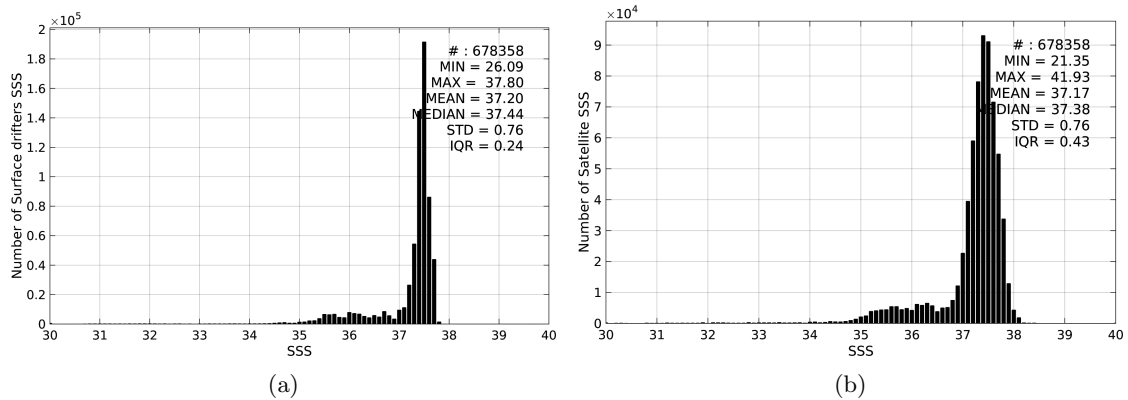
Figure 2: Histograms of SSS from Surface drifters (a) and SMOS-L3-CATDS-CECOS-LOCEAN-V2-9DAYS-25KM (b) considering all match-up pairs per bins of 0.1 over the Amazon and Orinoco river plumes Pi-MEP region and for the full satellite product period.
