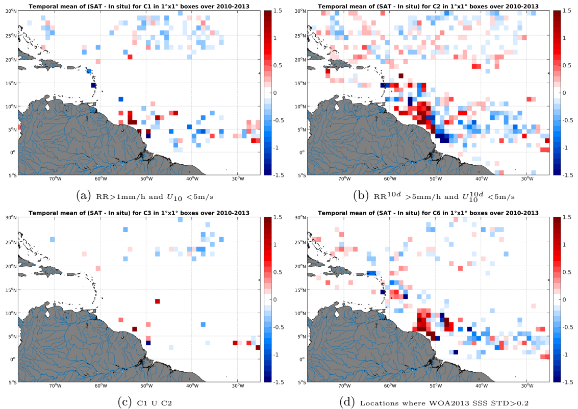
Figure 11: Temporal mean gridded over spatial boxes of size 1^\circ \times 1^\circ of \Delta SSS (SMOS-L3-CATDS-CECOS-LOCEAN-V2-9DAYS-25KM - Surface drifters) for 4 different subdatasets corresponding to:RR>1mm/h and U_{10} < 5 m/s (a), RR^{10d} > 5 mm/h and U_{10}^{10d} < 5 m/s (b), C1 U C2 (c),Locations where WOA2013 SSS STD>0.2 (d).
