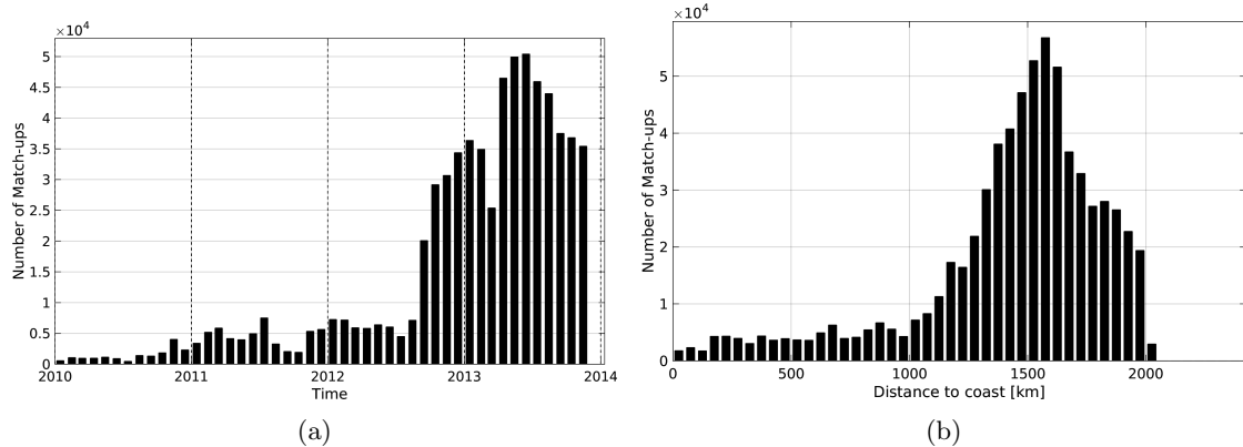
Figure 1: Number of match-ups between Surface drifters and SMOS-L3-CATDS-CECOS-LOCEAN-V2-9DAYS-25KM SSS as a function of time (a) and as function of the distance to coast (b) over the Amazon and Orinoco river plumes Pi-MEP region and for the full satellite product period.
